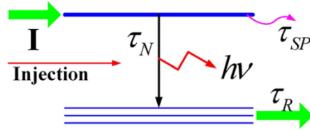
Fig(1): Simplified carrier dynamics model[12]
