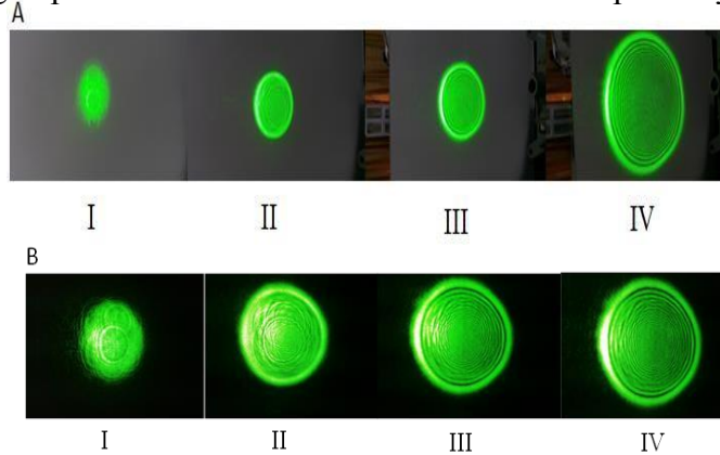
Fig (4). Variation of rings number in (A) paprika oil [ I : 3.8 mW , II: 15.2 mW , III: 30.4 mW , IV: 68.4 mW] and (B) pepper oil [ I: 7.4 mW , II: 29.6mW , III: 66.6mW, IV: 81.4 mW ] using light beam of \lambda = 532 nm against input power.
