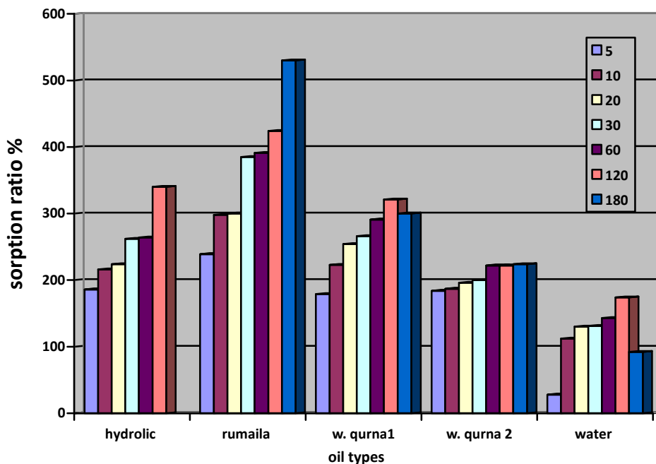
Fig (4) the variation of sorption ratio with oil types
