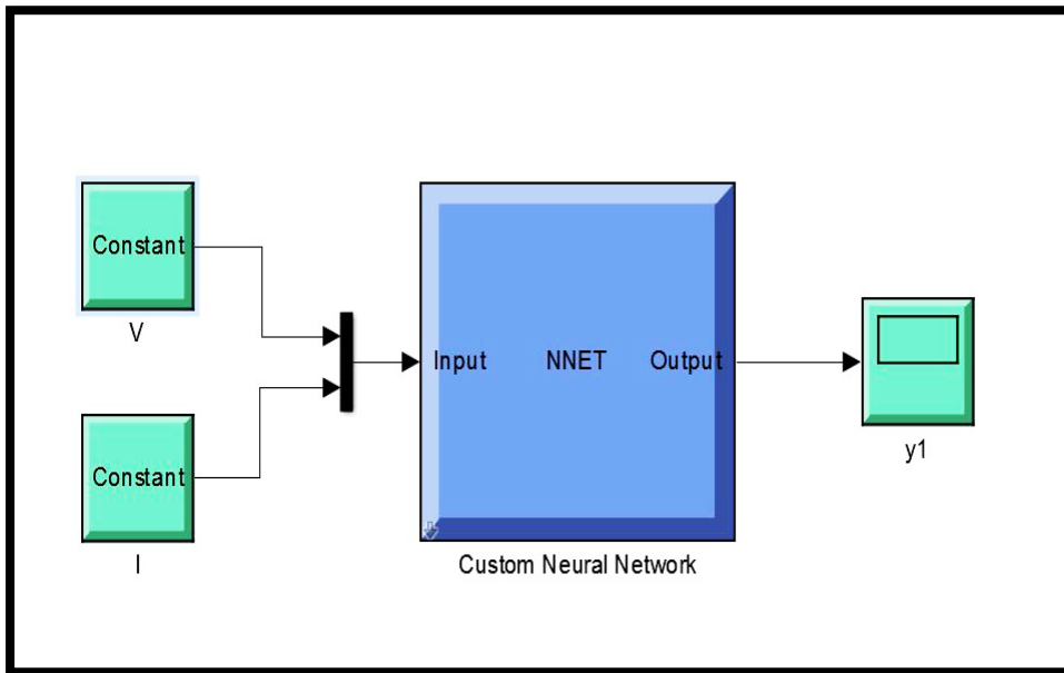
Figure 3: Deploy Neural Network Simulink Diagrams. [The Math Works, Inc., MATLAB R2015b].
