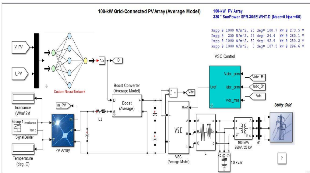
Figure 2: Photovoltaic system Simulink modeling (PV Array (Average Model)).
