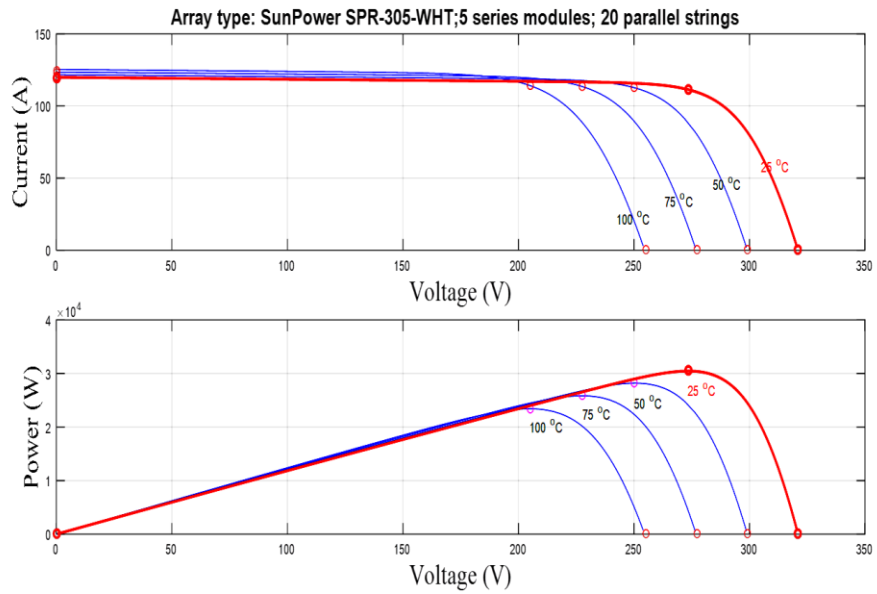
Figure 9: I - V and P - V Characteristics with Varying Operating Temperature.
