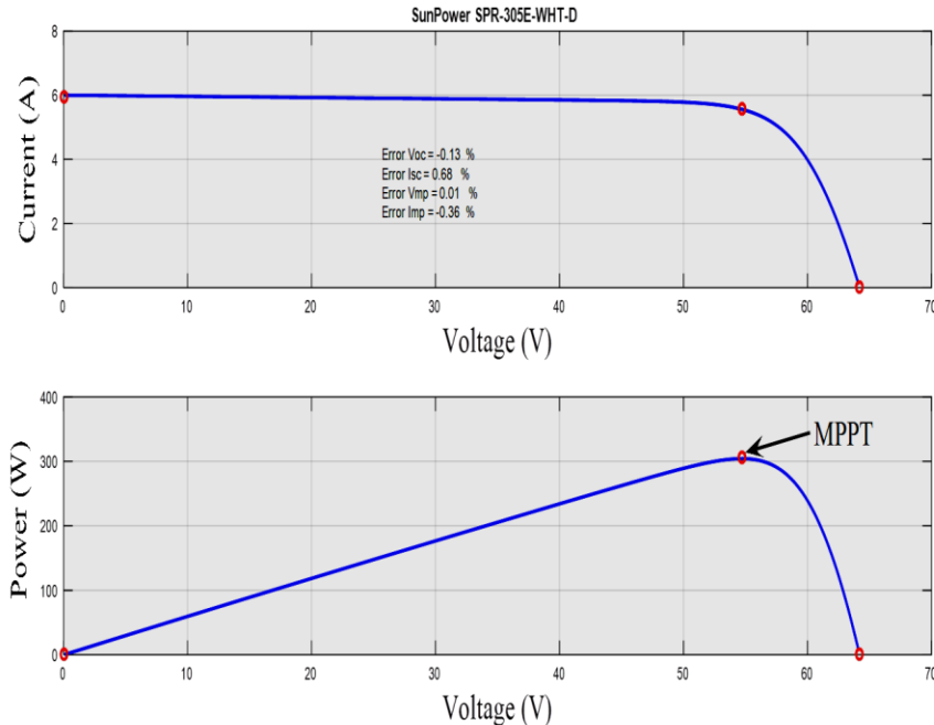
Figure 4 : I-V and P-V characteristics of the PV array modules show I_{sh} , V_{oc} , I_{mp} , V_{mp} , and MPPT.
