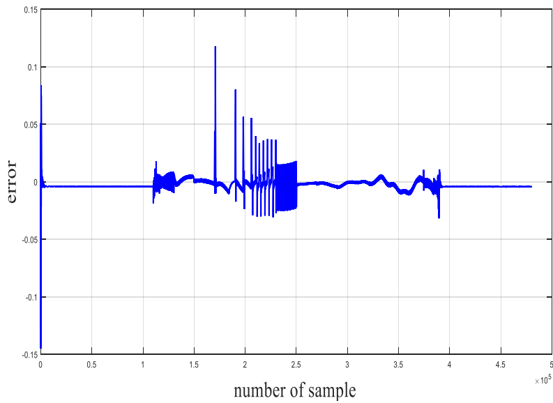
Figure 11: errors values of neural network.
