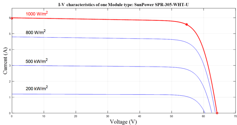
Figure 6: I-V characteristics of PV array with Varying Solar Irradiance Level of one module.
