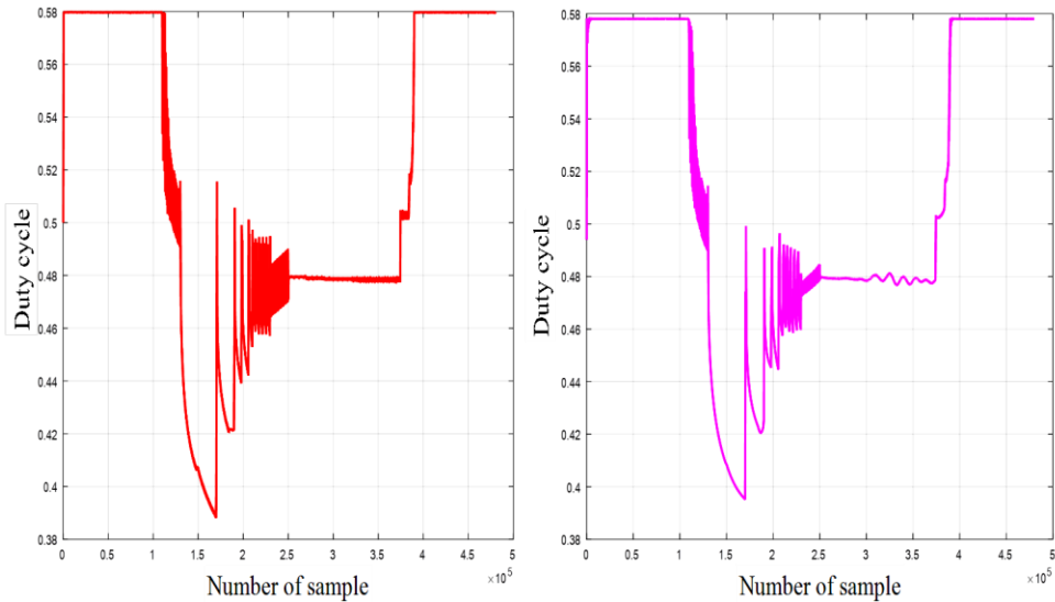
Figure 10a: Duty cycle of MPPT Controller MPPT Using perturb & Observe technique.
