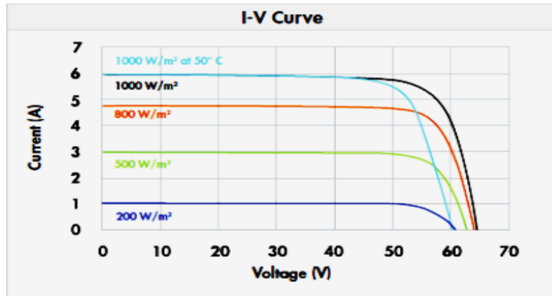
Figure 5: I-V characteristics of PV array with Varying Solar Irradiance Level Of one module [Antonio Faggio 2015] [17].
