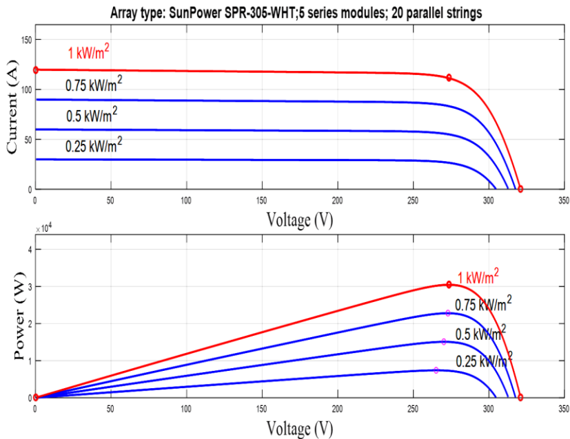
Figure 8: I-V and P-V characteristics of PV array with Varying Solar Irradiance Level.
