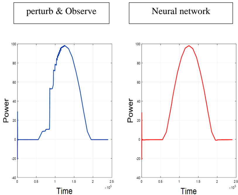
Figure 13: Power curve simulation result within 24 hours.
