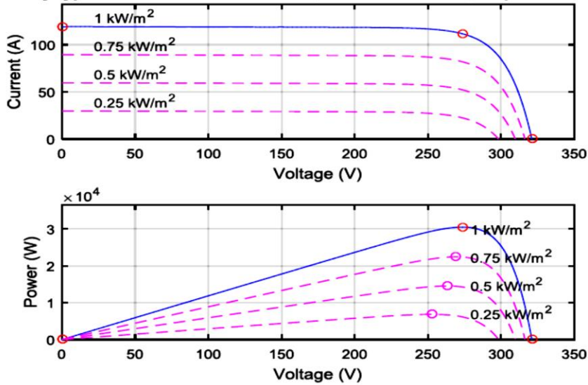
Figure 7: I-V and P-V characteristics of PV array with Varying Solar Irradiance Level of 5 series modules; 20 parallel strings [Antonio Faggio 2015] [17].
