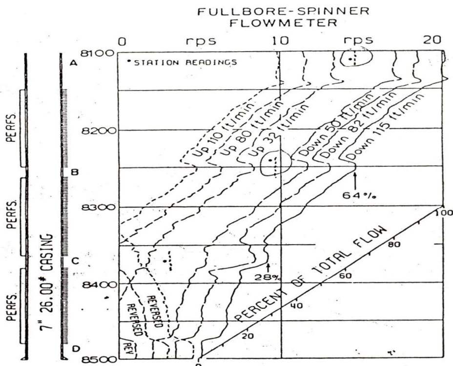
Fig. (1) Fullbore-spinner Flowmeter in a dump-flood
