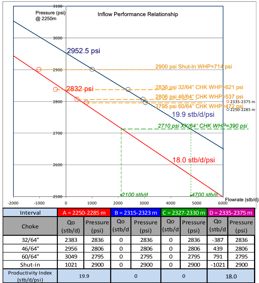
Fig.(8) Inflow Performance Relationship.
