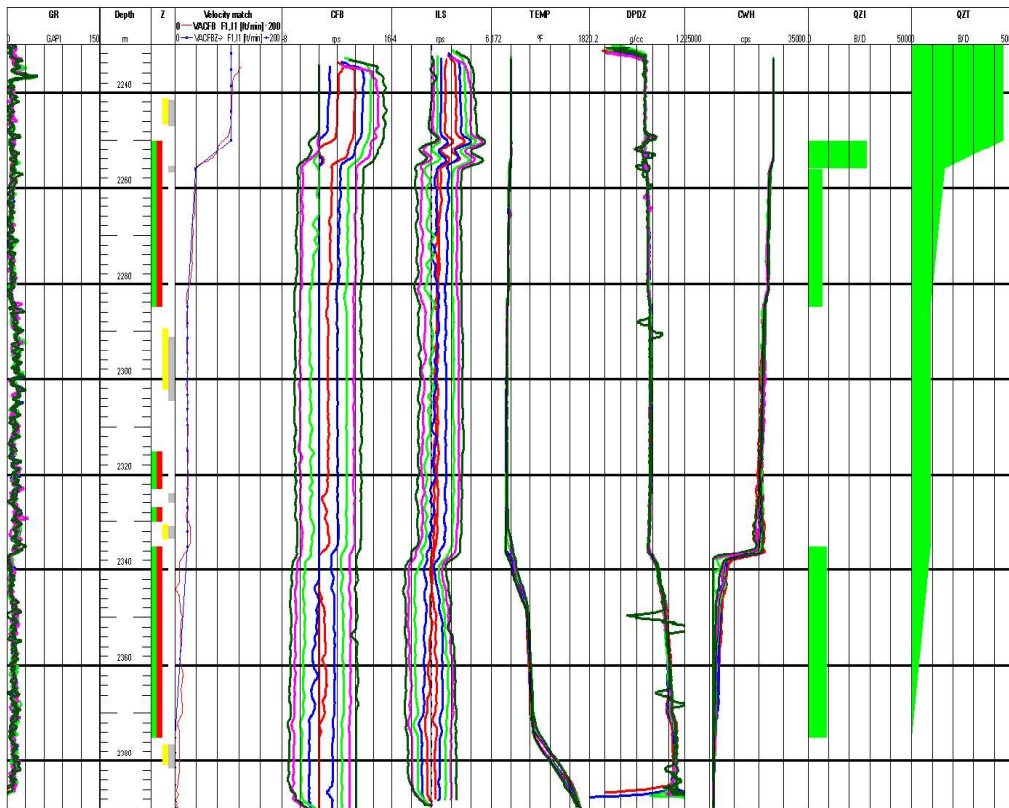
Fig. (3) Production Log-Processing Results (Flowing Choke .60/64")
