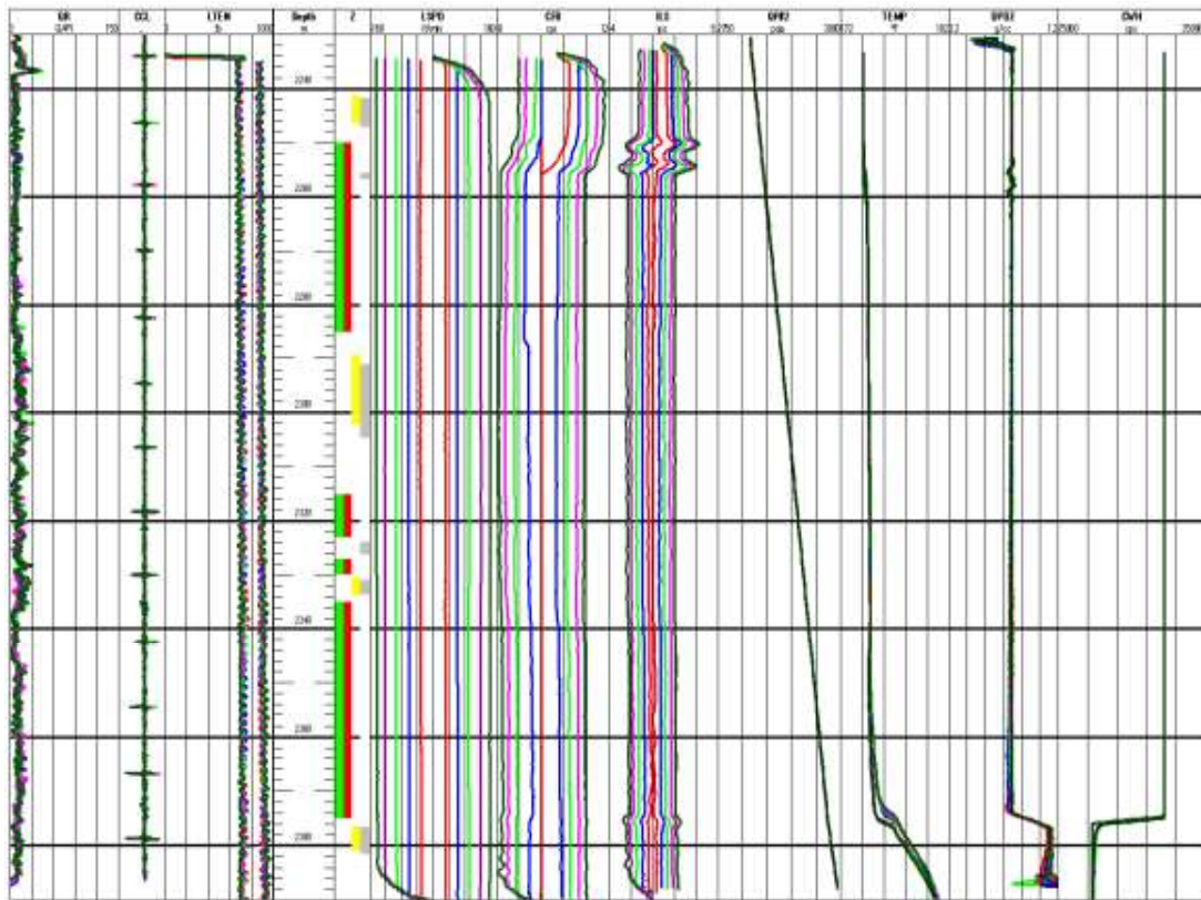
Fig.(7) Production Log-Processing Results (Flowing Choke 32/64").
