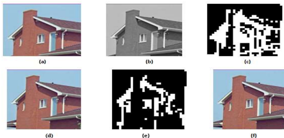
Figure (4): Simulation results using proposed system using different threshold values.(a) Original image, (b) Y Band, (c) Partition Band in correlated block (black) and uncorrelated block (white)(d) Recovered image with PSNR= 41.26 and CR=29.12 at Q_0=0.8, Q_1=2.5, \alpha=2, \beta=0.5, q_1=1, q_2=1, q_3=1 and T=15 , (e) Partition Band in correlated block (black) and uncorrelated block (white) and (f) Recovered image with PSNR= 42.86 and CR=18.01 at Q_0=0.8, Q_1=2.5, \alpha=2, \beta=0.5, q_1=1, q_2=1, q_3=1 threshold=30.
