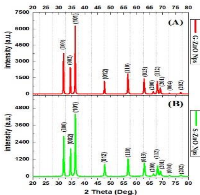
Figure 3: XRD spectra of (A) G-ZnO NPs and (B) S-ZnO NPs
