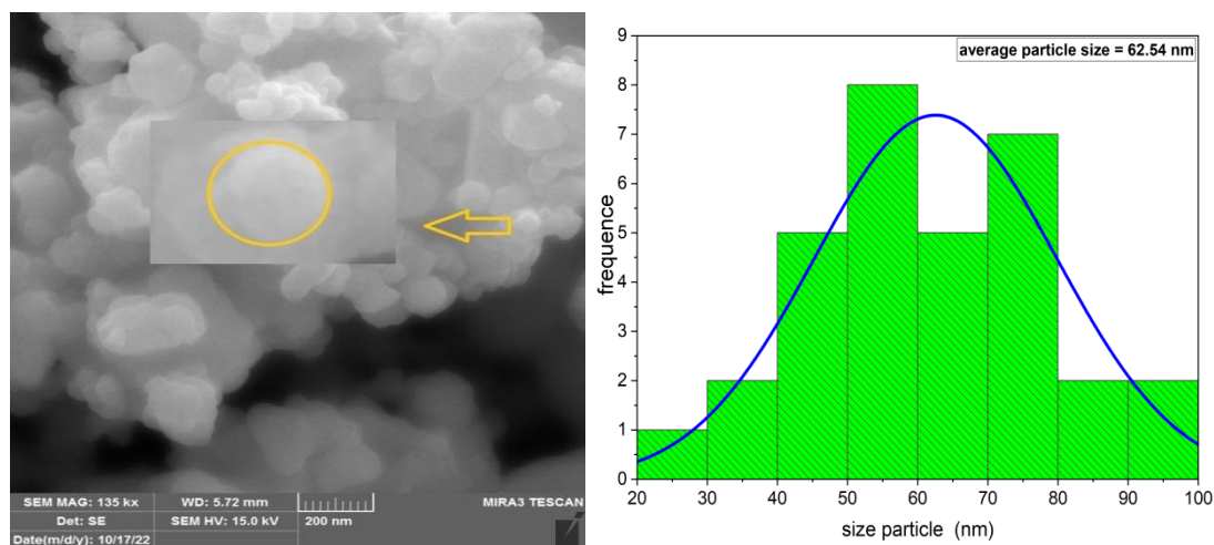
Figure 9: SEM micrograph of the synthesized G-ZnO NPs and composition using EDX.
