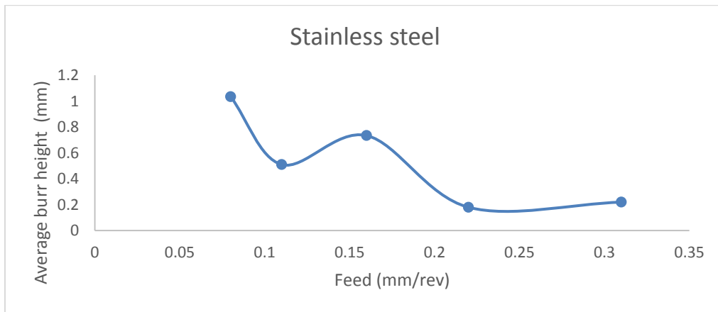
Figure. (9) Effect of feed on the average burr height in drilling stainless steel at cutting speed = 9.8 m/min.
