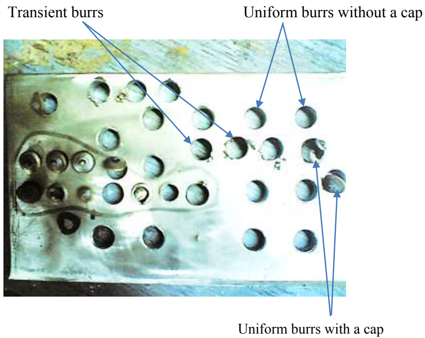
Figure. (4): Photographic view of drilling burrs in stainless steel.
