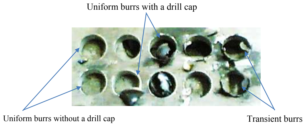
Figure (5): Photographic view of drilling burrs in low carbon steel
