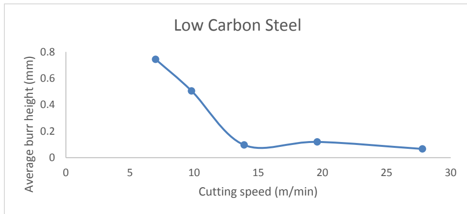
Figure. (8) Effect of cutting speed on the average burr height in drilling low carbon steel at feed = 0.31 mm/rev.
