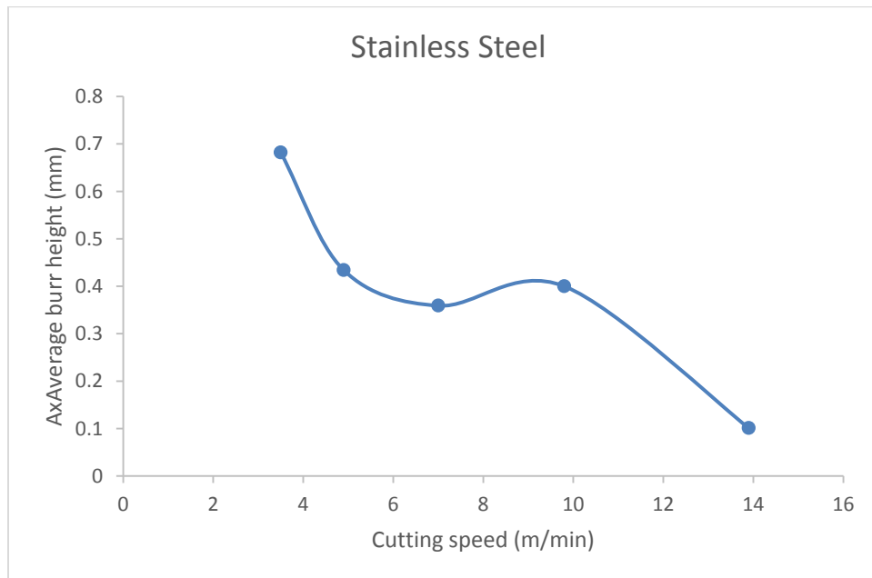
Figure. (7) Effect of cutting speed on the average burr height in drilling stainless steel at feed = 0.16 mm/rev.
