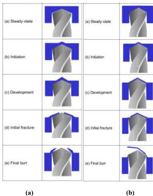
Figure. (3) Burr formation mechanism stages of (a) a uniform burr and (b) a crown burr in drilling AISI 304L [11]
