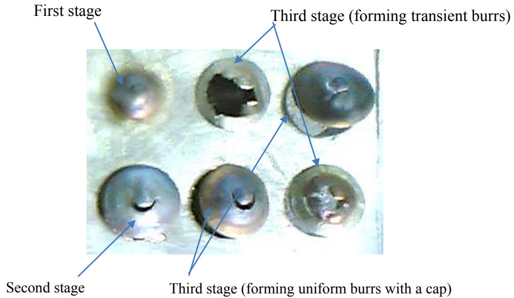
Figure. (6): Photographic view of burr formation mechanisms of transient and uniform burrs in drilling low carbon steel and stainless steel.
