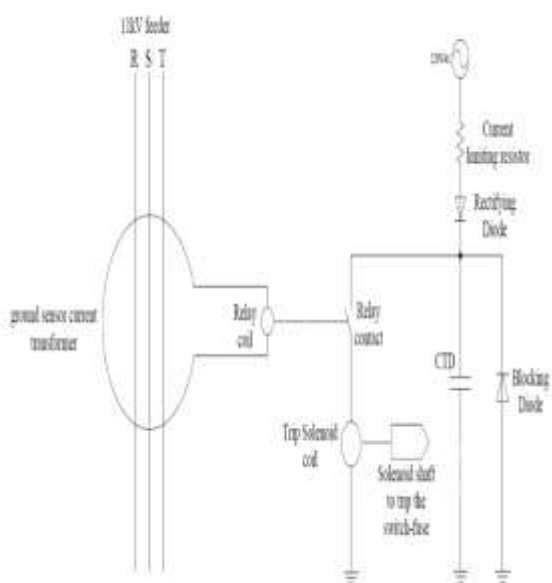
Figure 11: A diagram representing switch-fuse control circuit.
