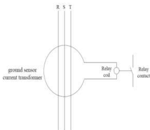
Figure 10: Relay operated by ground sensor current transformer
