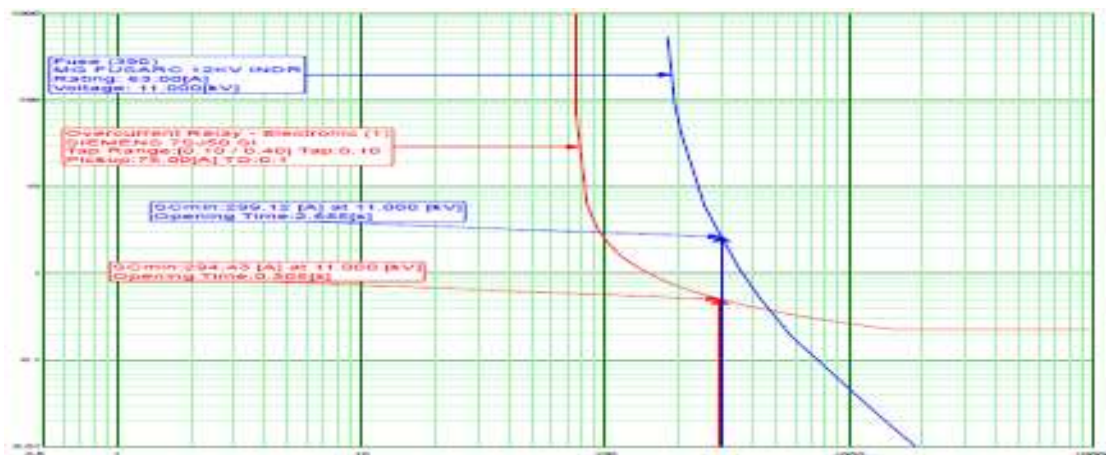
Figure 7: the “time – current” characteristics of both the relay and the HRC fuse
