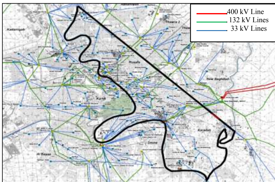
Figure 1: Electrical distribution network of Al-Rusafa General Directorate
