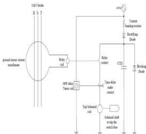
Figure 12: A diagram representing switch-fuse control circuit with time delay
