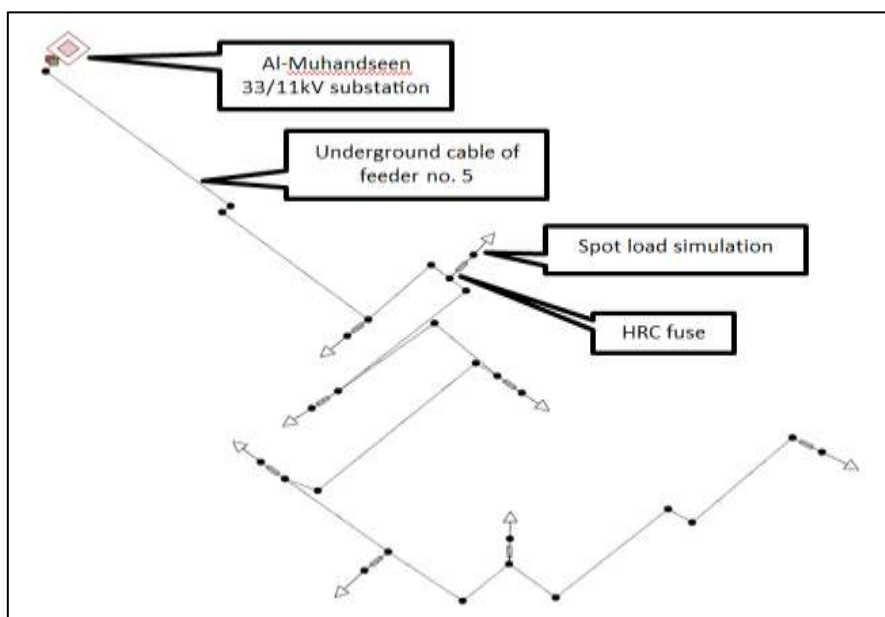
Figure 2: layout of feeder no.5 from Al-Muhandseen Substation (33/11 kV)
