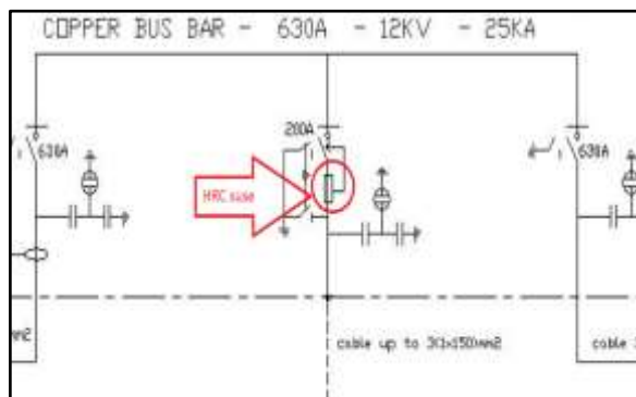
Figure 3: Single line diagram of the high voltage compartment [2]
