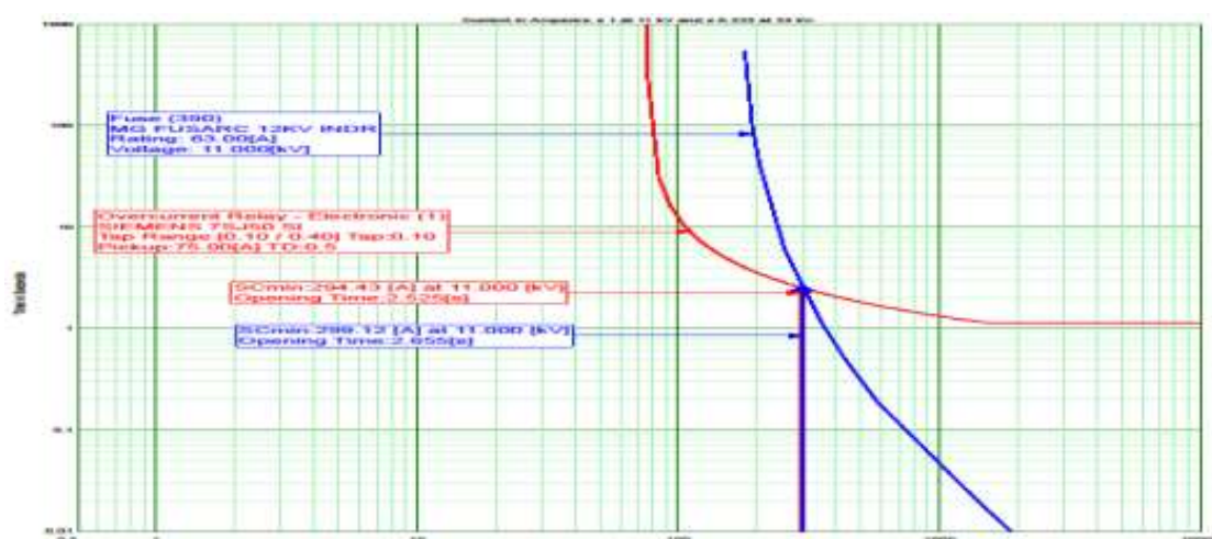
Figure 8: Branch device coordination for case (a)
