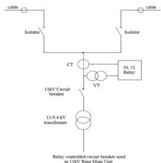
Figure 9: Ring main unit with circuit breaker instead of switch-fuse
