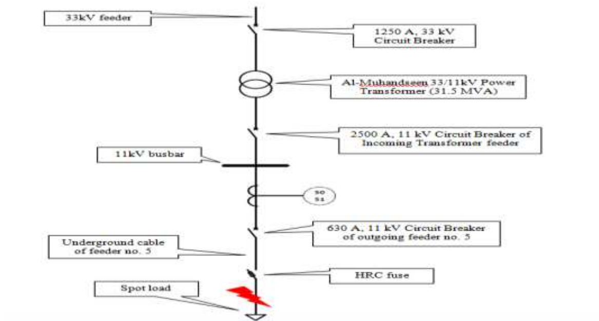
Figure 6: the network under coordination
