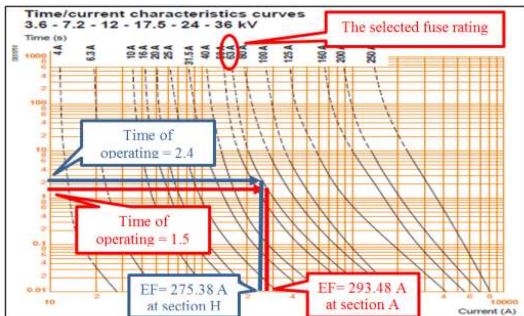
Figure 4: The maximum and minimum earth fault currents at the first and last section of the feeder and the corresponding time of operation of the HRC fuses
