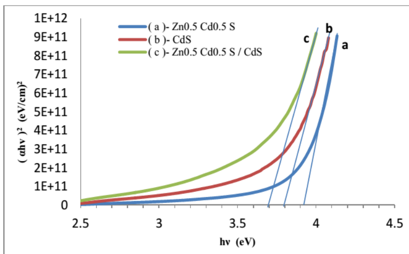
Figure 5: Optical energy gap of nanocrystalline thin films (a)- \text{Zn}_{0.5}\text{Cd}_{0.5}\text{S} , (b)- \text{CdS} and (c) - \text{Zn}_{0.5}\text{Cd}_{0.5}\text{S} / \text{CdS}
