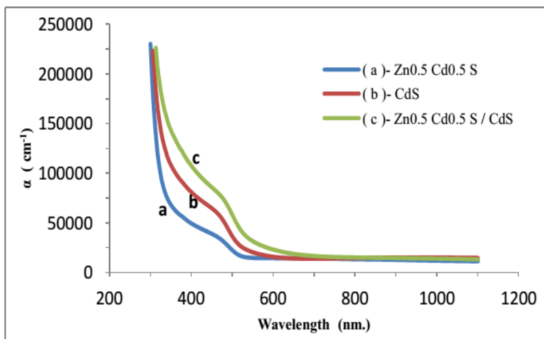
Figure 4: Absorption coefficient of nanocrystalline thin films versus wavelength (a)- \text{Zn}_{0.5}\text{Cd}_{0.5}\text{S} , (b)- \text{CdS} and (c) - \text{Zn}_{0.5}\text{Cd}_{0.5}\text{S} / \text{CdS}
