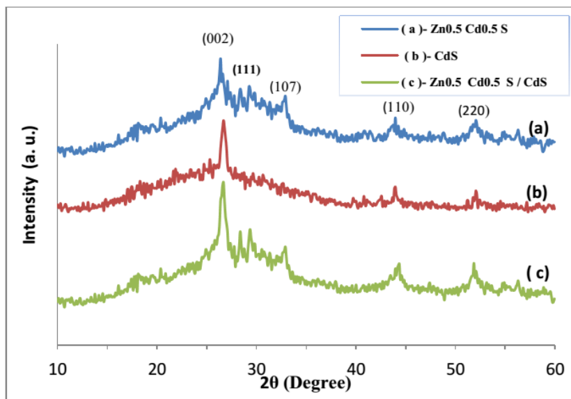
Figure 1: XRD spectra of nanocrystalline thin films (a)- \text{Zn}_{0.5}\text{Cd}_{0.5}\text{S} , (b)- \text{CdS} and (c)- \text{Zn}_{0.5}\text{Cd}_{0.5}\text{S} / \text{CdS} .
