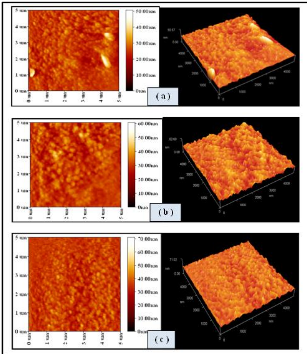
Figure 2: AFM images of nanocrystalline thin films with 2 dimension and 3 dimension. ( a)- \text{Zn}_{0.5}\text{Cd}_{0.5}\text{S} , ( b)- \text{CdS} and ( c ) - \text{Zn}_{0.5}\text{Cd}_{0.5}\text{S} / \text{CdS}
