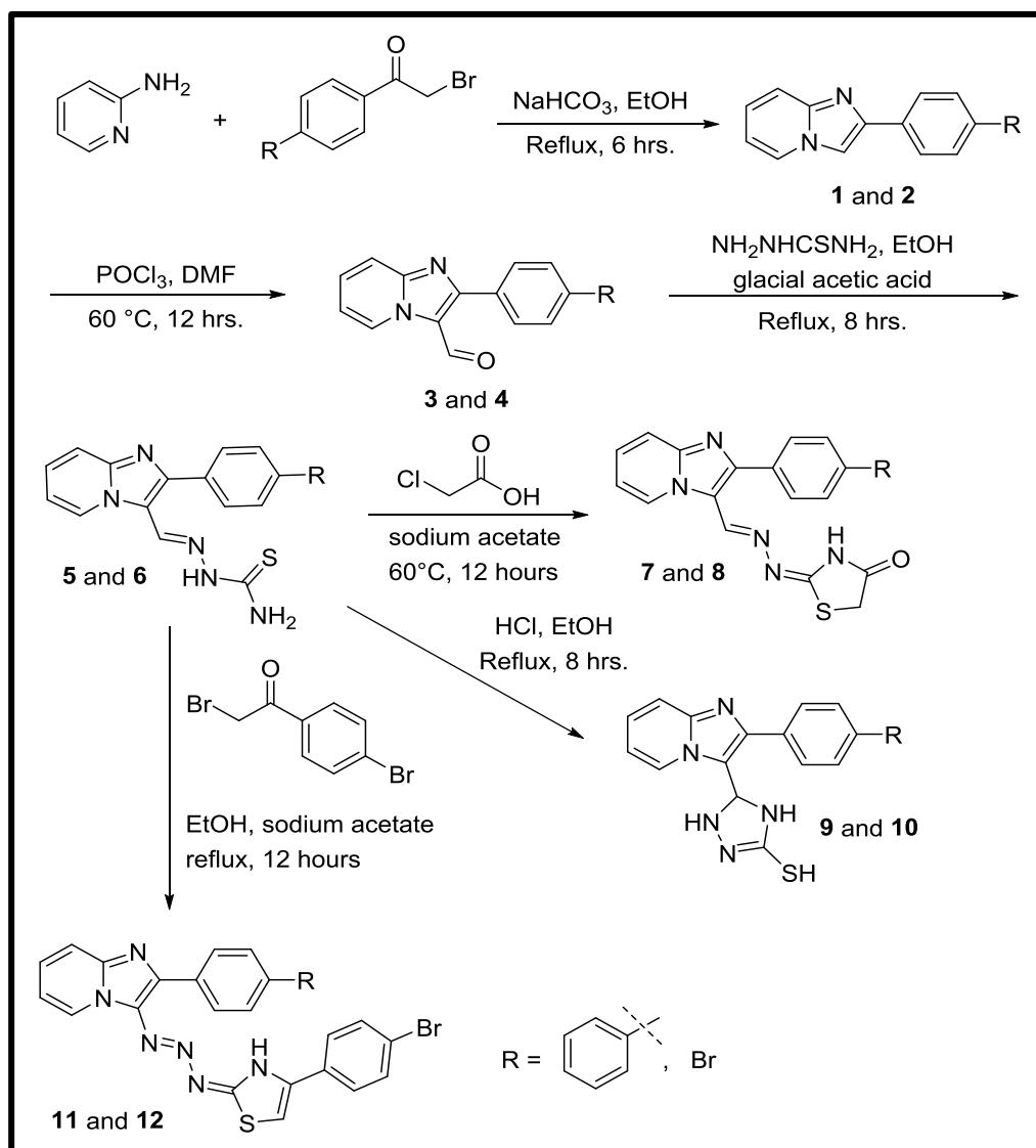
Scheme 1: The synthetic route of the products 1-12
