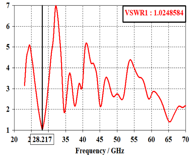
Figure 18: VSWR of proposed antenna at config.2.
