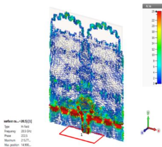
(a) State-1 at 28.5 GHz.
