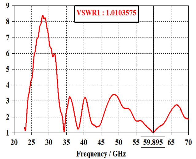
Figure 17: VSWR of proposed antenna at config.1.
