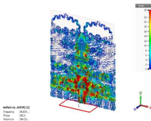
(a) State-1 at 38.8 GHz
