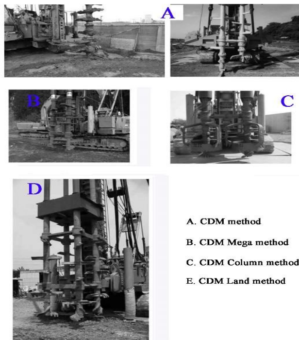
Figure 6. Several kinds of CDM included mixing shafts and blades (Photo is a courtesy of the Cement DMM Association)[6]
