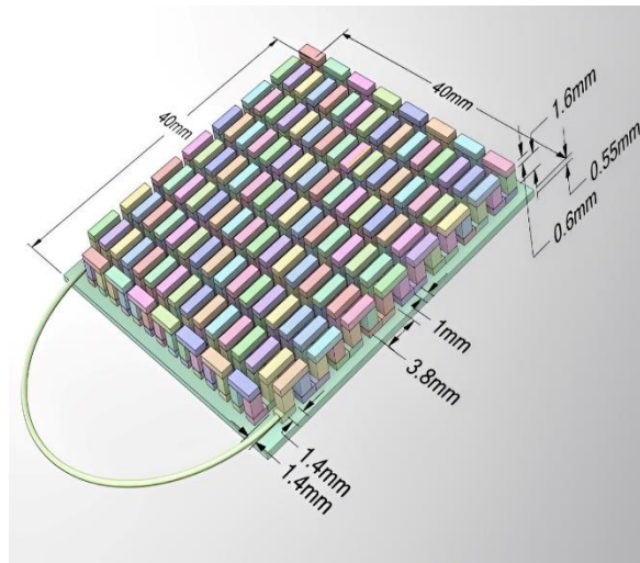
Figure 2. The entire thermoelectric generator consists of 127 thermocouple pairs [11].
