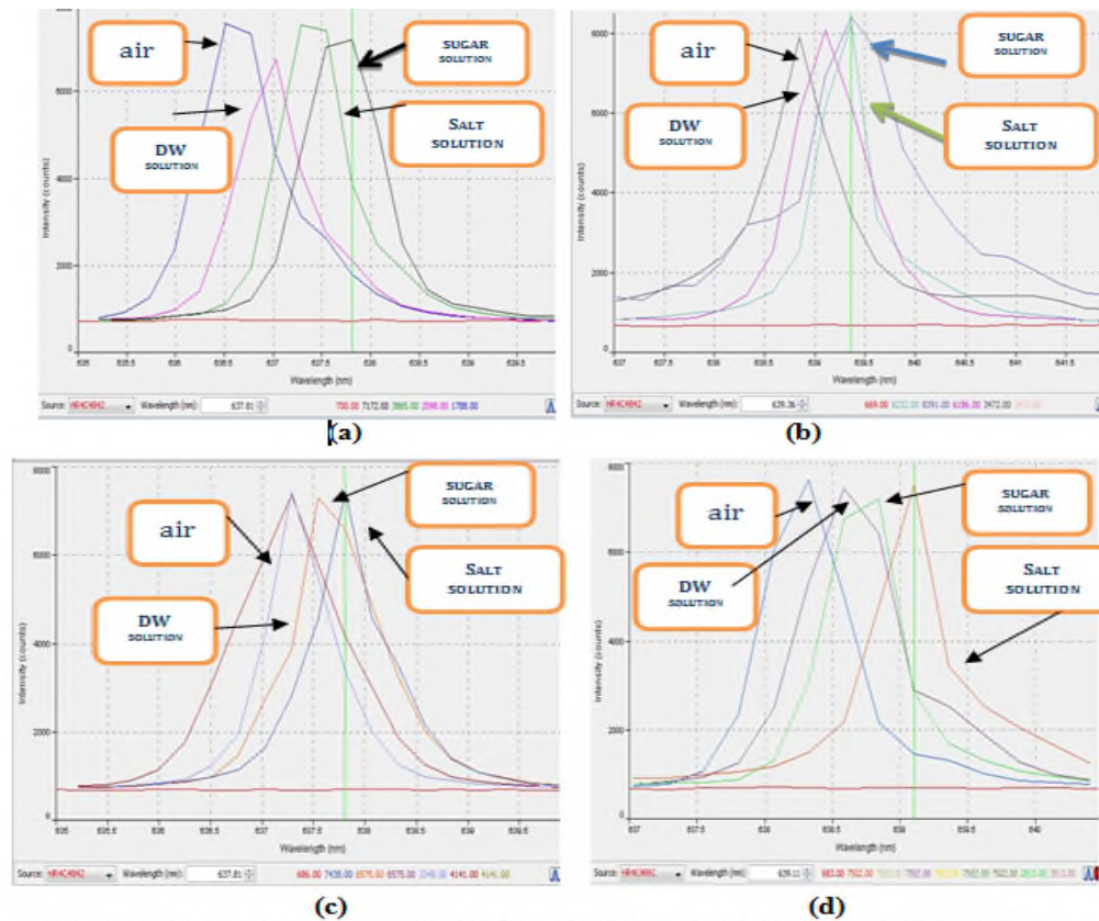
Figure(4) Sensor response based on LSPR localized in air, DW, sugar solution and salt solution. (a,b) for SMF splice with MMF at the first day prepared the Cu NPs solution and after a week respectively ,(c,d) for SMF splice with SMF at the first day prepared the Cu NPs solution and after a week respectively.
