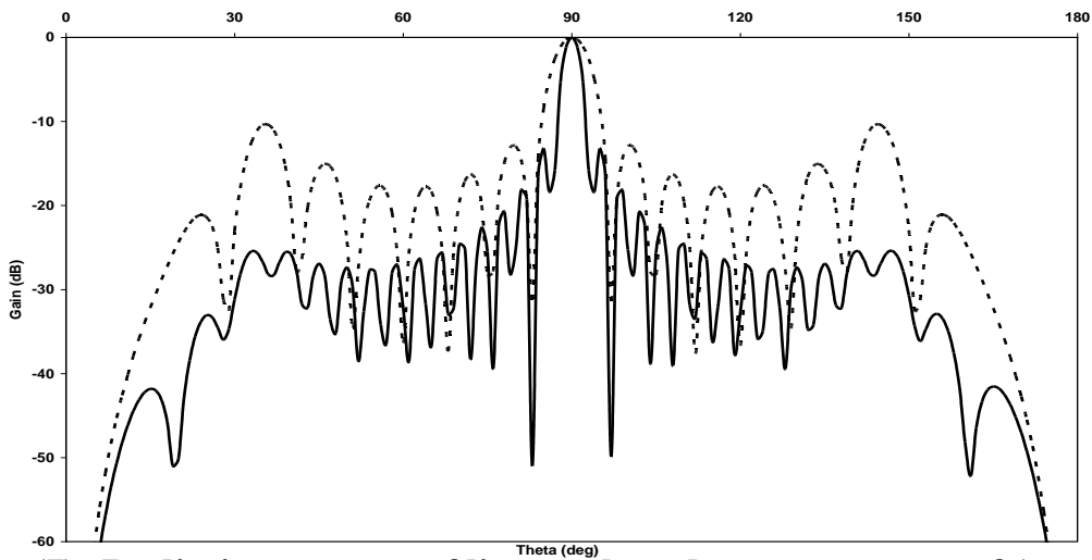
Fig.(7): Radiation pattern of linear phased array antenna of (.....)16 slots and (—) of 32 slots spaced by 0.5\lambda .
