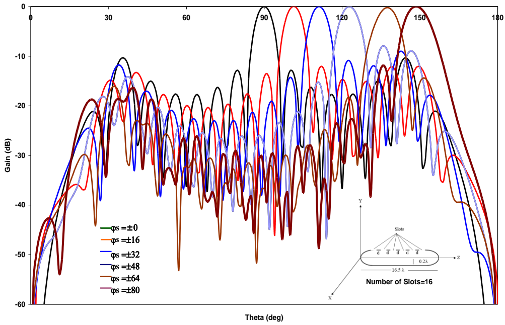
Fig.(6): Radiation pattern of linear phased array antenna of 16 slots of 0.5\lambda w.r.t steering angle.
