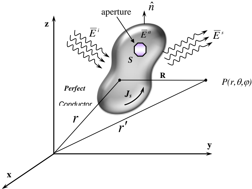
Fig.(2): the general radiation problem
