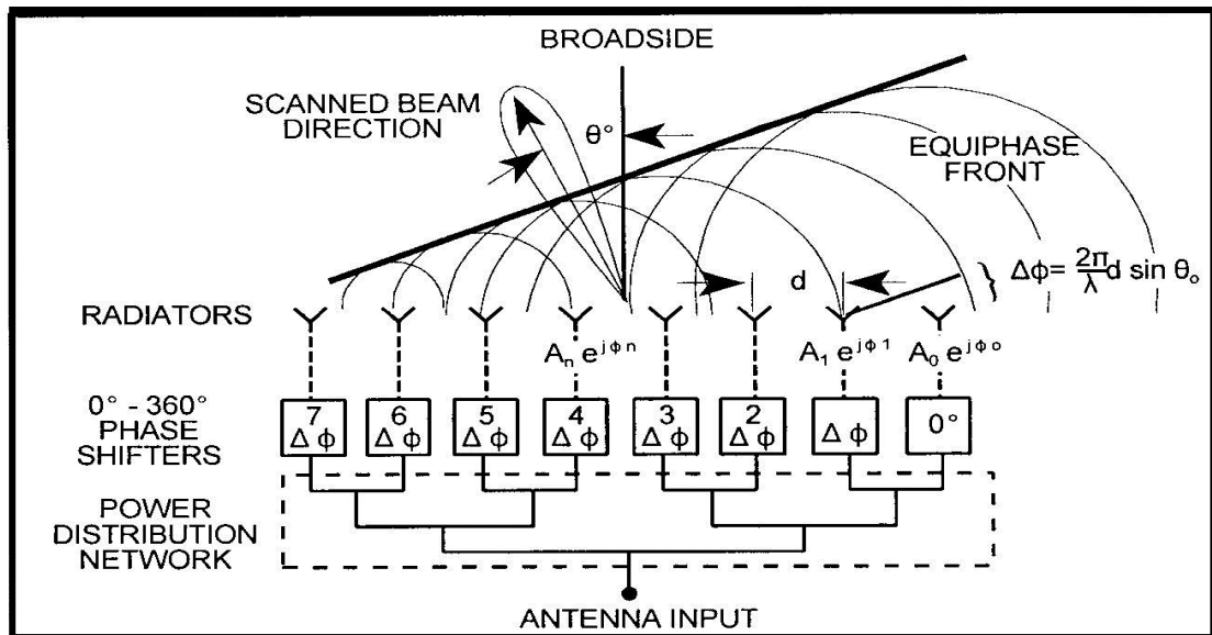
Fig.(5) : linear phased array antennas with corporate fed.
