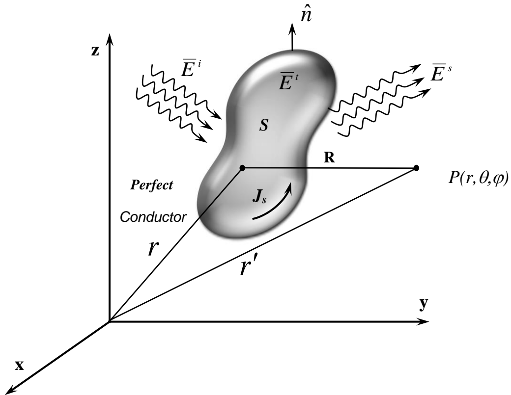
Fig.(1): the general scattering problem
