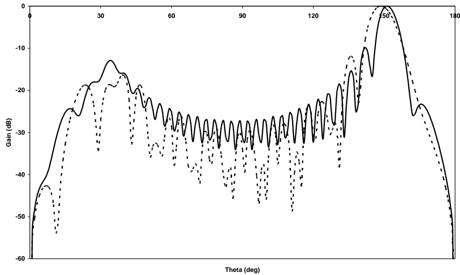
Fig.(8): Radiation pattern of linear phased array antenna of 16 slots (.....) and (—) of 32 slots of 0.5\lambda with steering angle (a) 16^\circ , (b) 32^\circ , (c) 48^\circ , (d) 64^\circ , and (e) 80^\circ .
