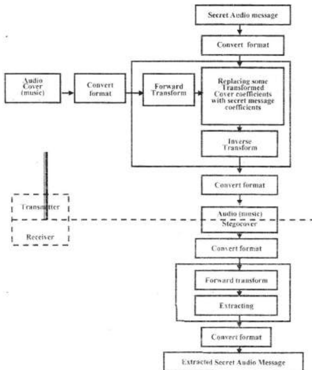
Figure (1) Block Diagram of Proposed Algorithm
