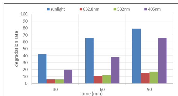
Fig. (8): Comparison of the degradation rates of MB dye with nanostructured ZnO catalyst under sunlight and three different lasers wavelengths.
