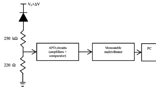
Fig.(2): Schematic diagram for generating random numbers based on dark counts of single-photon avalanche photodiodes [6]
