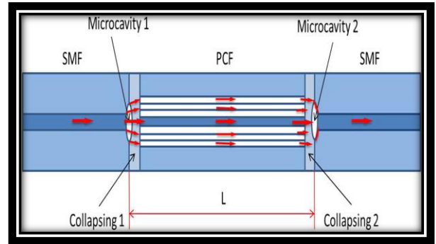
Fig. (4): Micro-cavity formation at the splicing point between SMF (on the left) and SCPCF (on the right) [16].
