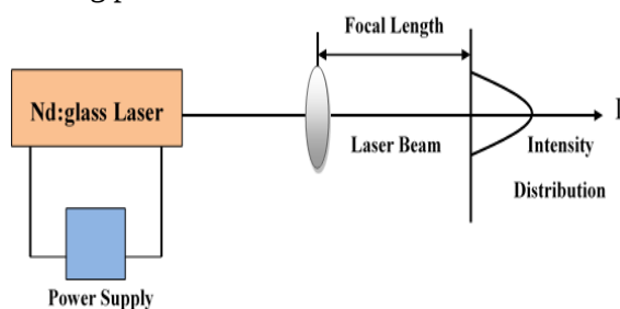
Fig. (1): The essential features of Nd:Glass laser.
