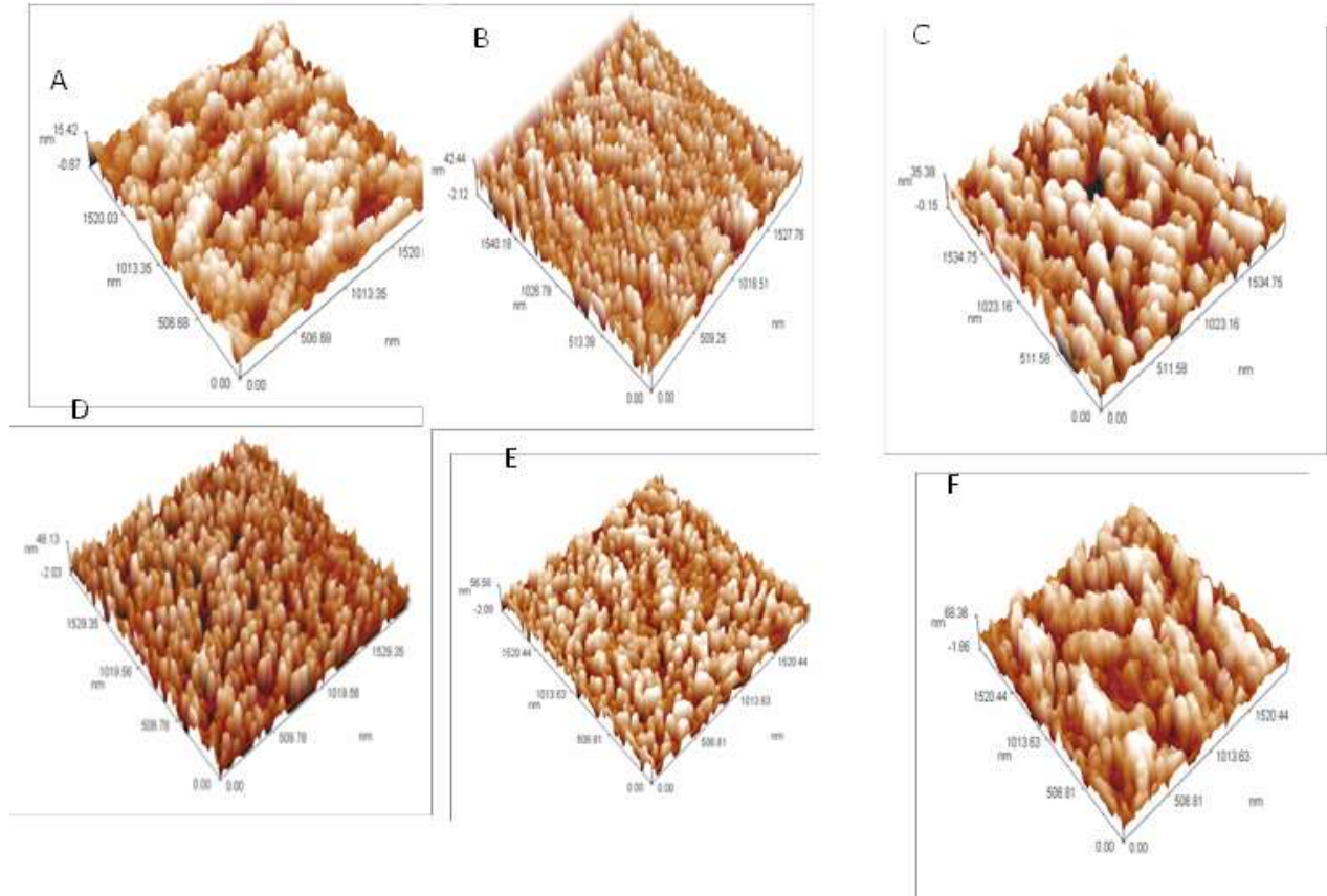
Figure (5): (3-dimentional AFM pictures). A. Untreated specimen ( R_a = 3.05 nm). Er,Cr:YSGG laser treated specimens: B. (20 s / 60 \mu s / 4 W) R_a = 7.73 nm, C. (30 s / 60 \mu s / 4 W) R_a = 8.88 nm, D. (40 s / 60 \mu s / 3.5 W) R_a = 10.2 nm, E. (20 s / 700 \mu s / 3.5 W) R_a = 12.4 nm, F. (30 s / 700 \mu s / 3.5 W) R_a = 14.5 nm
