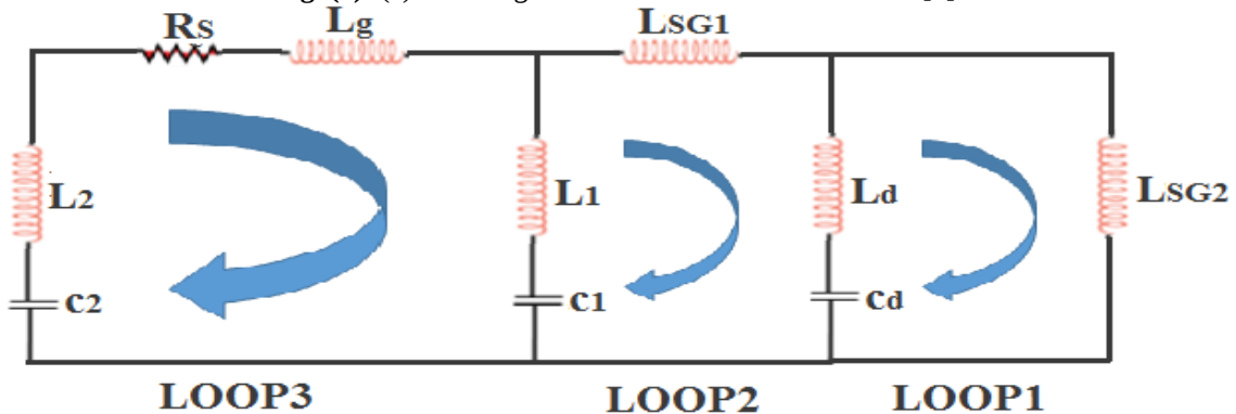
Fig. (2): (b) (TSBC) equivalent Blumlein line circuit [7], where:
