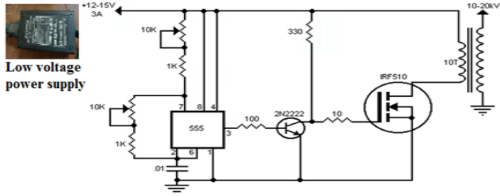
Fig. (1): High voltage power supply circuit diagram [7]
