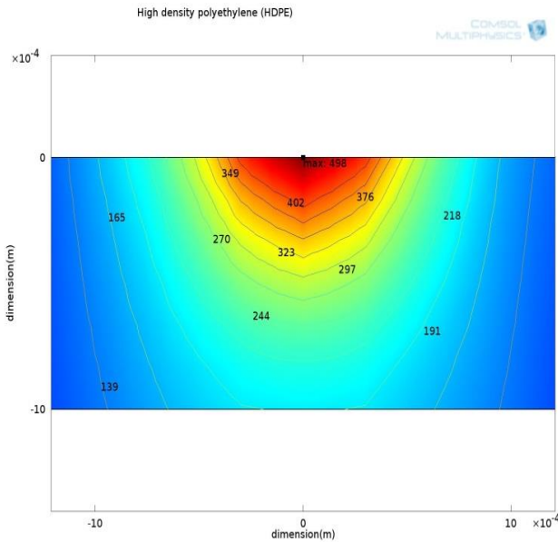
Fig.11 Temperature distribution simulated at 5J energy, pulse duration 9.9 ms, and 0.5 kW peak power.
