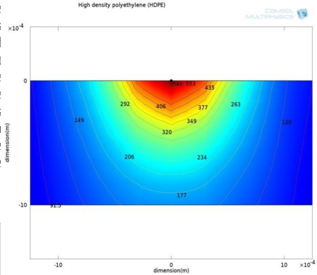
Fig 13 Temperature distribution simulated at 5J energy, pulse duration 4 ms and 1.2 kW peak power.
