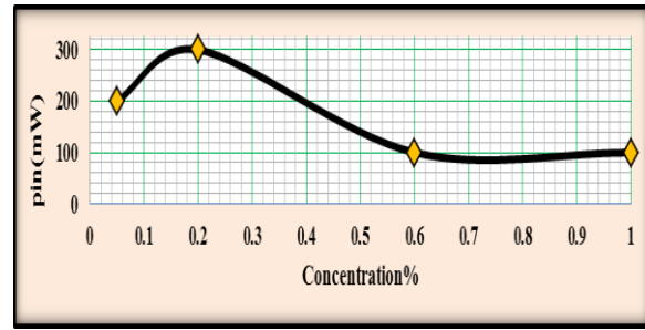
Fig (7): start sensing powers of 532nm CW diode laser with different Ag/D.I. water nanofluid concentrations.
