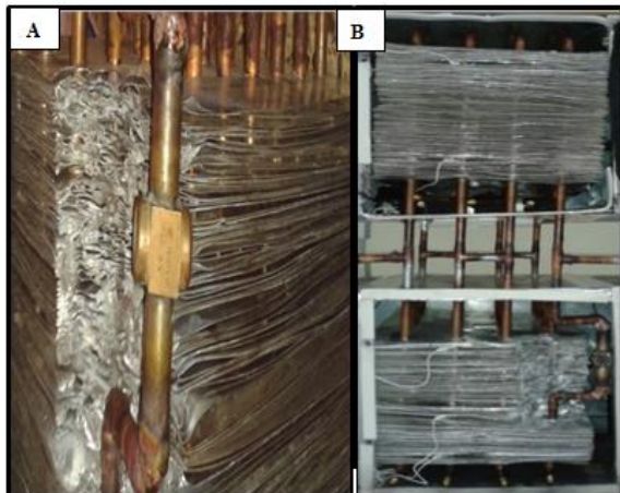
Fig (1: A, B ): HPHE with windows.(A) Side view of connecting windows with HPHE, (B) HPHE contains windows in the evaporator section.
