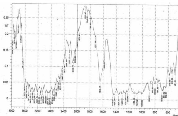
Fig.2: FTIR spectra for GNPs with Rh-6G and NaCl emptied on paper
