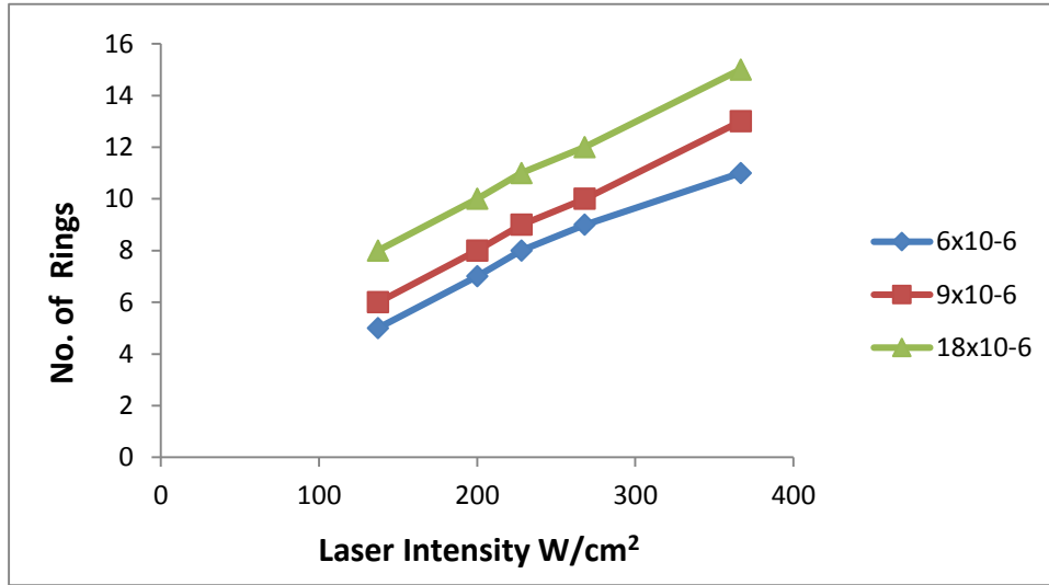
Fig. 6: The number of diffraction rings formed using( F-MWCNTs/Ag NPs) acetone suspension at various volume fraction irradiated by various laser intensities.
