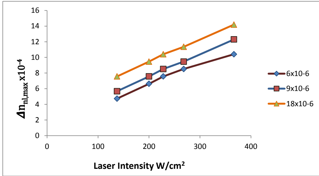
Fig. 8: The maximum change of F-MWCNTs/Ag-NPs acetone suspension at volume fraction value of 6 \times 10^{-6} , 9 \times 10^{-6} and 18 \times 10^{-6} .
