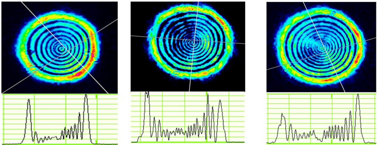
Fig.7: The self-diffraction pattern rings generated by using F-MWCNTs /Ag-NPs acetone hybrid nano-fluid at volume fraction of 6 \times 10^{-6} , 9 \times 10^{-6} and 18 \times 10^{-6} respectively at laser power density 228 W/cm².
