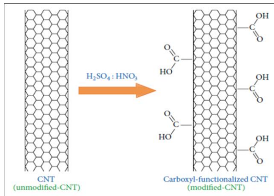
Fig. 1: Scheme of the chemical functionalization of a MWNT.
