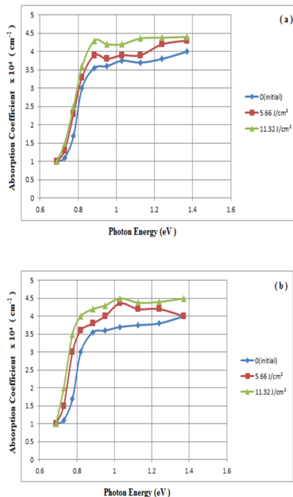
Fig.(5): The curves of absorption coefficient ( \alpha ) vs ( h\nu ) of the samples; (a)Vacuum Environment , (b) Water Environment
