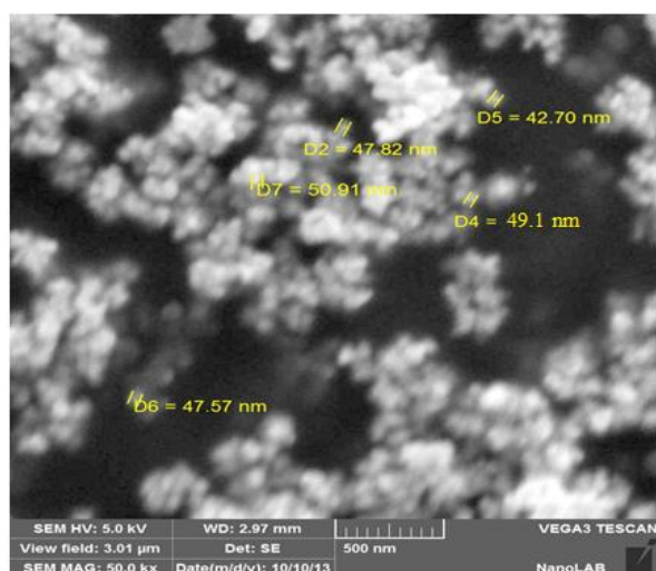
Fig. (1): Scanning electron microscopy image for Pd NPs at room temperature (25 ^\circ\text{C} ).
