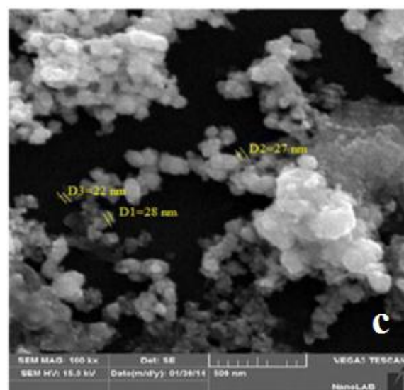
Fig. (1): Scanning electron microscopy image for Pd NPs at room temperature (25 ^\circ\text{C} ).
