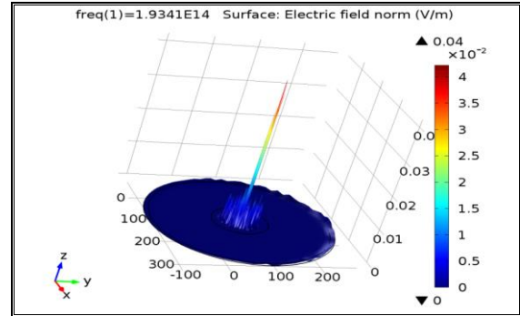
Fig. (5): (f)laser beam profile that exist from PCF(LMA-10) of taper waist diameter =60 \mu m with immersed in the external solution with refractive index 1.38
