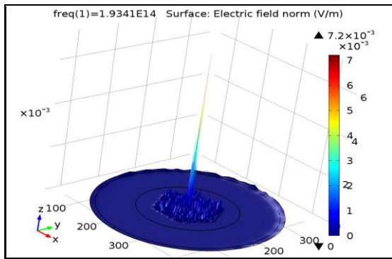
Fig. (5): (c)laser beam profile that exist from PCF(LMA-10) of taper waist diameter =107 \mu m with immersed inthe external solution with refractive index 1.38 .
