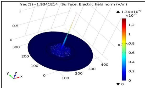
Fig. (5): (d)laser beam profile that exist from PCF(LMA-10) of taper waist diameter =90 \mu m with immersed in the external solution with refractive index 1.38.
