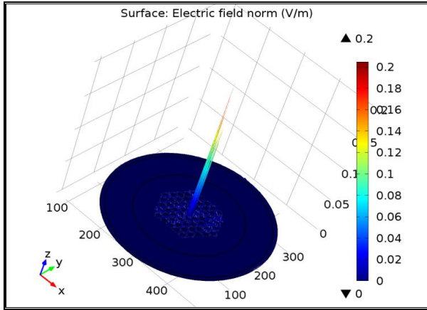
Fig. (5): (b) laser beam profile that exist from PCF(LMA-10) of taper waist diameter =125 \mu m with immersed in the external solution with refractive index 1.38
