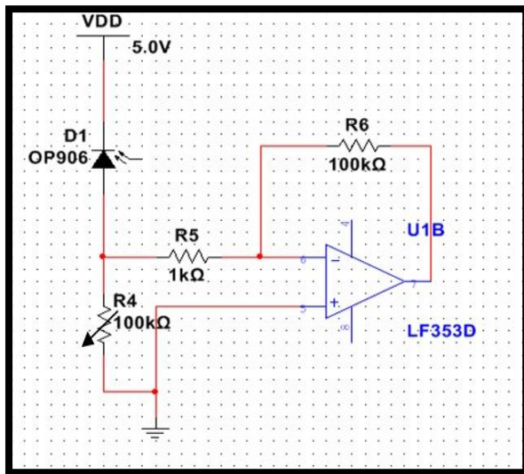
Figure 2 the photodetector simulation by electronic workbench.
