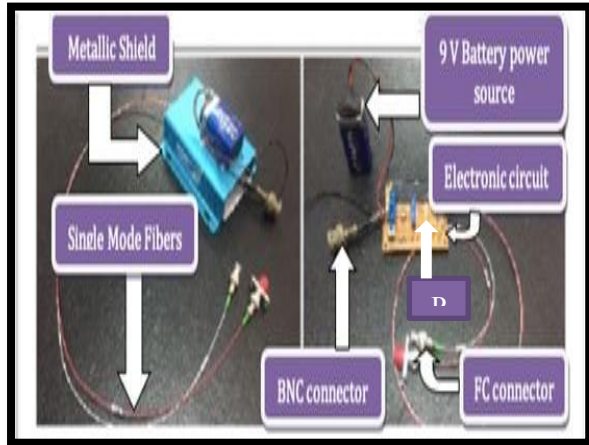
Fig. (4): Experimental setup of the photodetector circuit.
