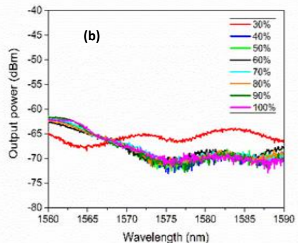
Fig. 3. The transmission spectra response of the OFHS as function of RH with NCF diameter of 125 \mu\text{m} .
