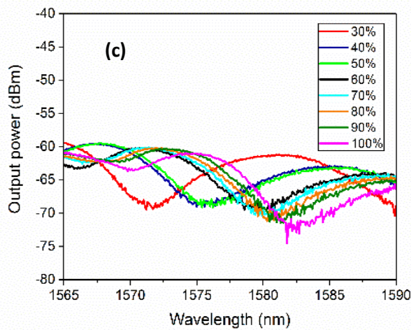
Fig. 4. The transmission spectra response of the RH sensor for different NCF diameter (a) 100 \mu\text{m} , (b) 80 \mu\text{m} and (c) 60 \mu\text{m} .
