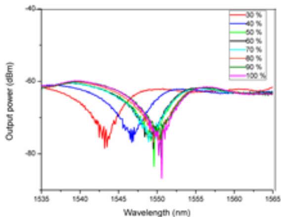
Fig. 3. The transmission spectra response of the OFHS as function of RH with NCF diameter of 125 \mu\text{m} .
