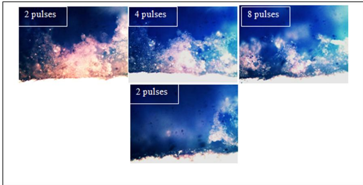
Fig. (2): Microscopic cross section image of iron plate cleaned with different number of Nd:YAG laser pulses and 9.17 \times 10^{10} \text{ W/cm}^2 laser intensity.
