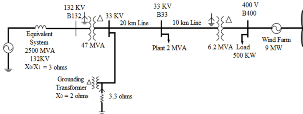
Figure (4) Single-line diagram of the wind farm connected to a distribution system
