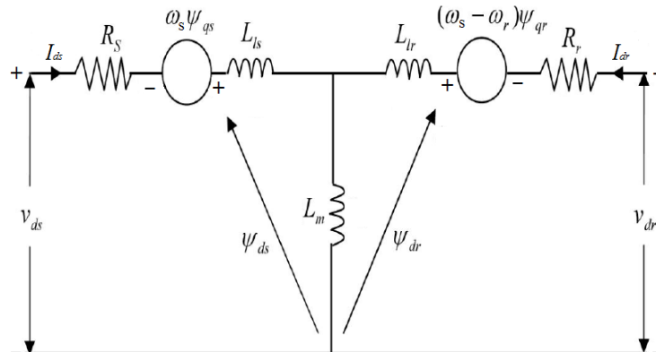
Figure (2) Dynamic d axis circuit
