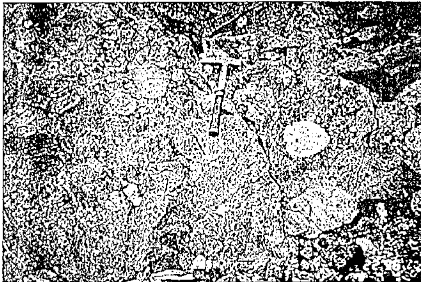
Figure 3. Field photos of the Conglomerate formation. Hammer is about 30 cm long.
