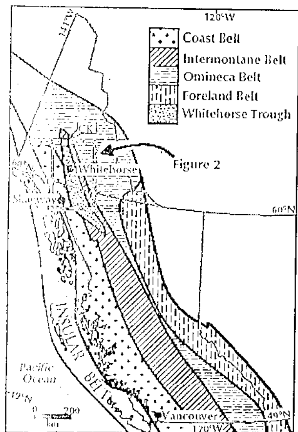
Figure 1. Morphogeological belts of the Canadian Cordillera (after Gabrielse et al., 1991), and location of the study area. CK = Carmacks sampling area.
