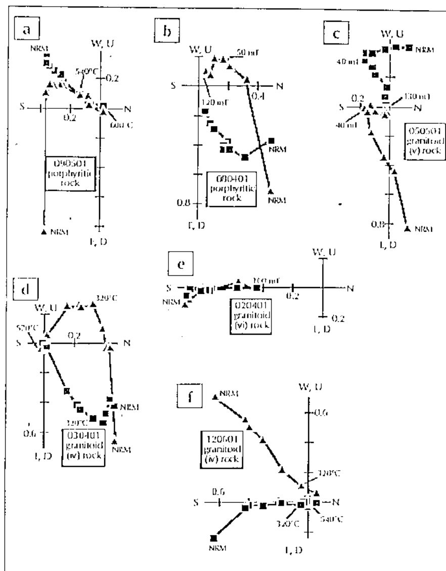
Figure 8. Orthogonal demagnetization plots (after Zijdeveld, 1967) with conventions the same as Figure 5.
