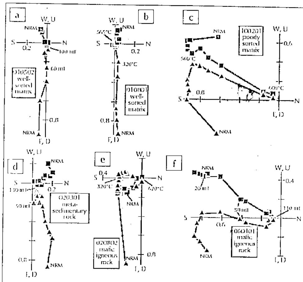
Figure 5. Orthogonal demagnetization plots (after Zijdeveld, 1967). Triangles are in the vertical plane, up-north-down-south (U-N-D-S) and the squares are in the horizontal plane, west-north-east-south (W-N-E-S).
