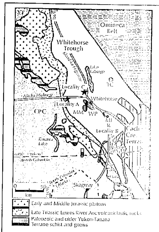
Figure 2. Tectonic map of the south-central Yukon and collections Localities (A, B and C) for the Conglomerate formation of the Laberge Group.
