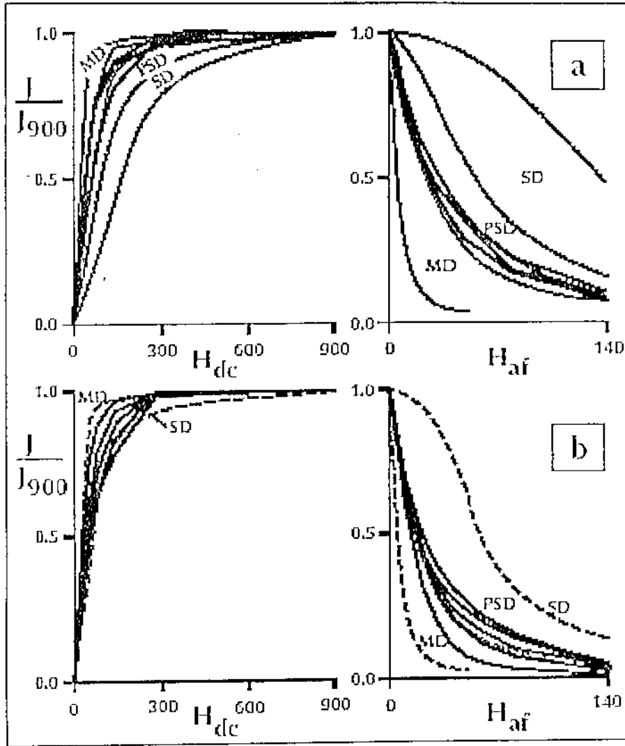
Figure 6. Representative SIRM acquisition and decay curves for (a) the matrix specimens and (b) the elast specimens. The horizontal axes represent the magnetization acquired ( H_{dc} ) and decayed ( H_{df} ), measured in mT, and the y-axis is the measured intensity as a ratio of the saturation intensity (at 900 mT). The reference curves in (a and b) are for multidomain (MD), pseudosingle domain (PSD), and single domain (SD) pyrrhotite and magnetite, respectively.
