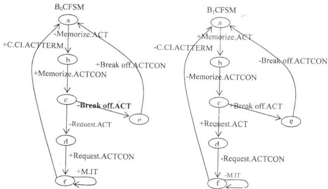
Fig. (19) CFSM model for integrated total application function in IEC870 protocol.
