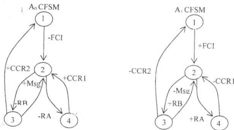
Fig. (18) CFSM model for Transmission of integrated total application function in ASEA protocol.
