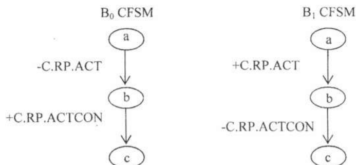
Fig (24) CFSM model for warm start function of re-start up application function in IEC870 protocol.
