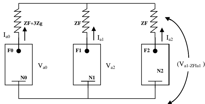
Fig(15) The final connection to networks sequence of fault (LLG)at a point (F)
