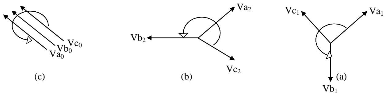
Fig(4) three phases group which symmetrical components to the system unbalanced
