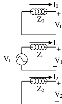
Fig(3) Thevenins equivalent for each sequence in fault location
