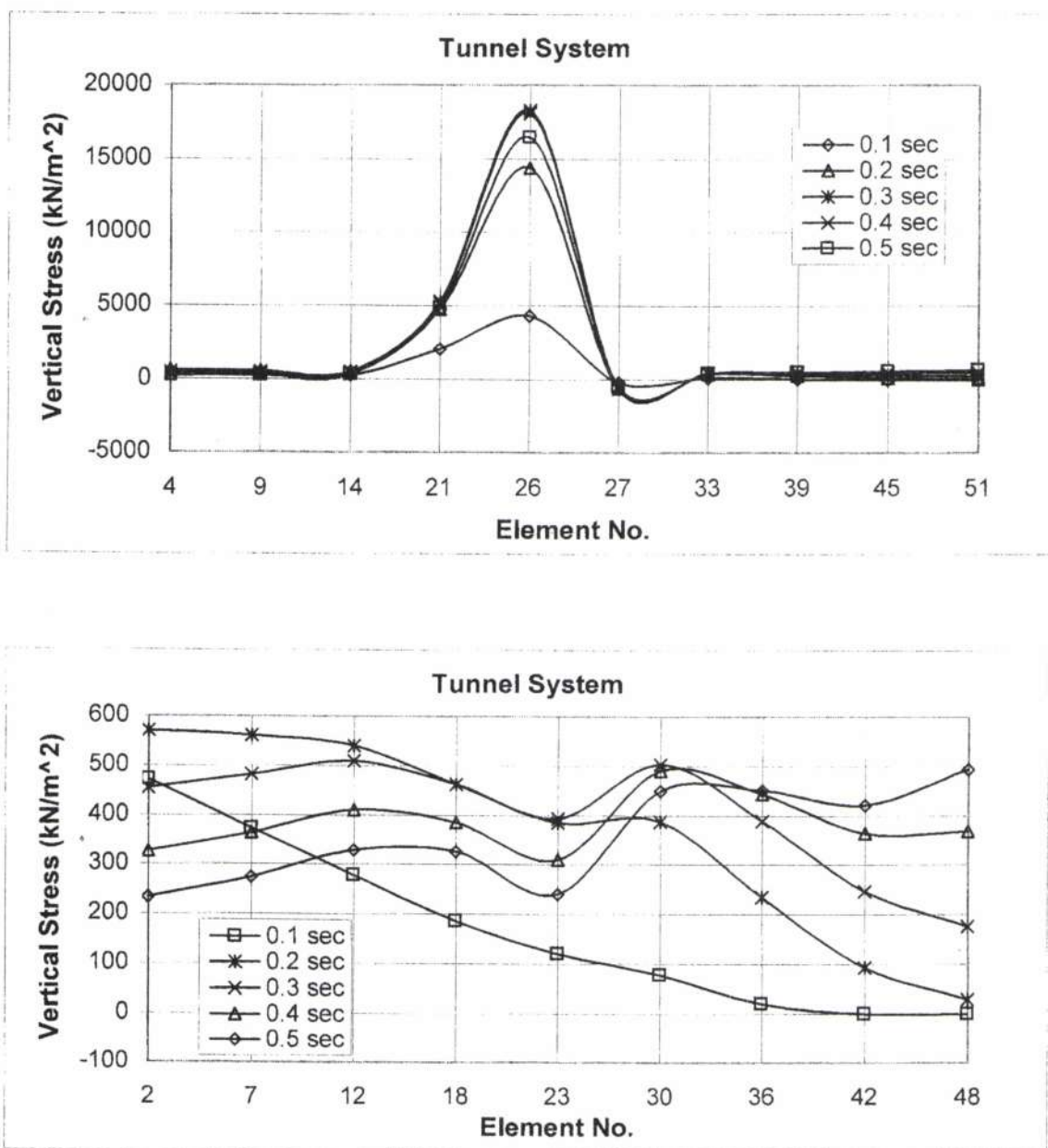
Fig. (5). Elastic Vertical Stresses in a 7 m Deep Tunnel System Due to Blast Loading.
