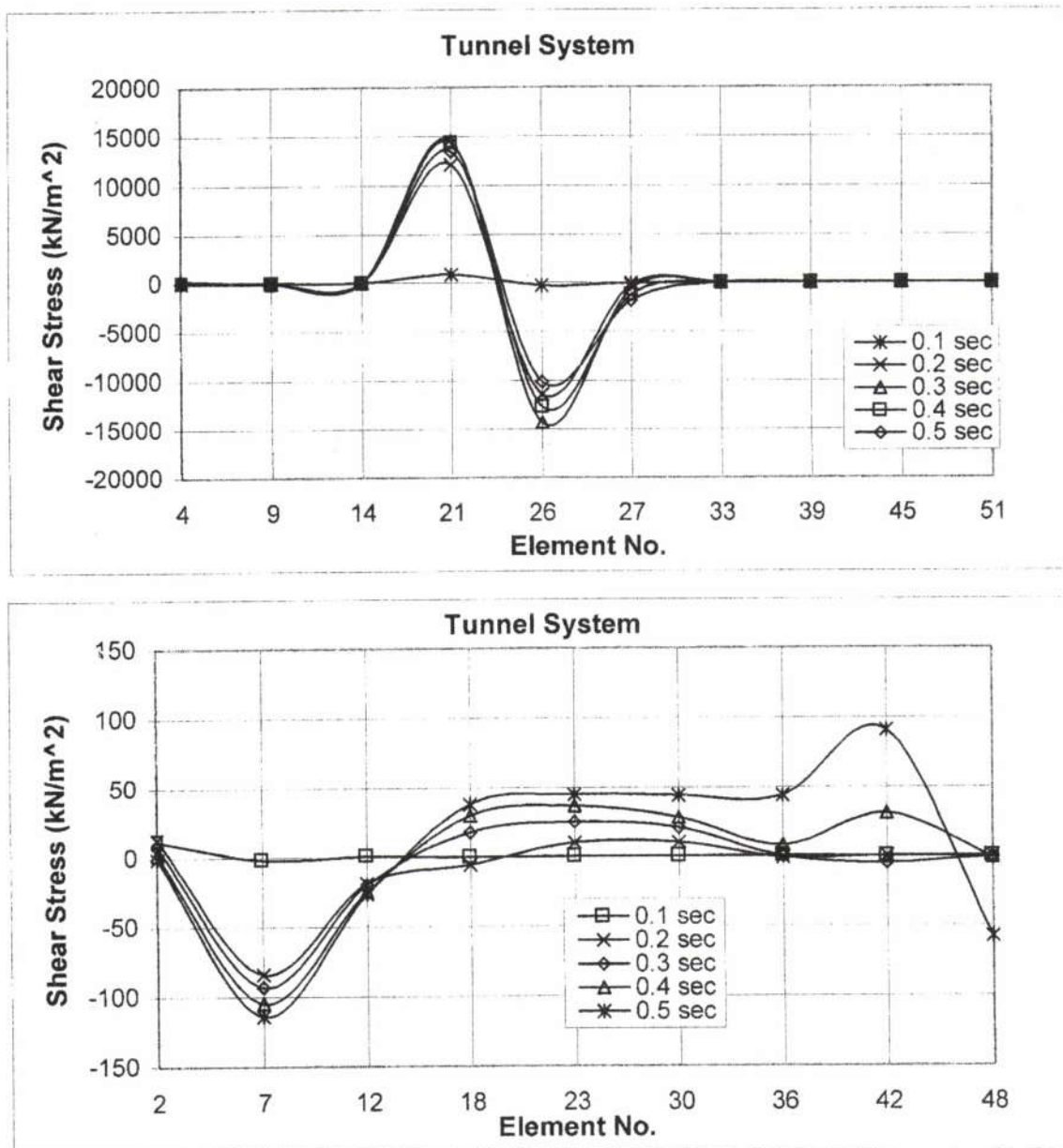
Fig. (12). Bounding Surface Model Stresses in a 7m Deep Tunnel System Due to Blast Load.
