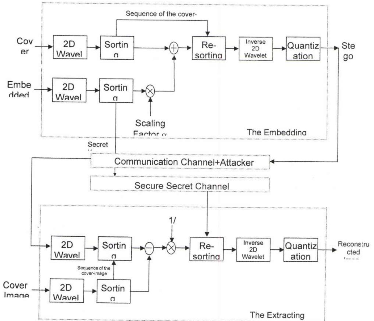
Fig. (1) The Proposed Stego-
