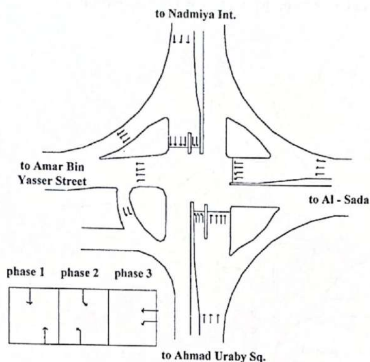
Fig. (9) Geometric layout, phasing plane fifth proposed layout obtained by this study
