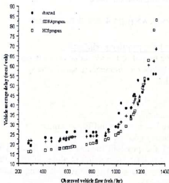
Fig. (2) Comparison between observed vehicle delay with that produced by SIDRA and HCS programs
