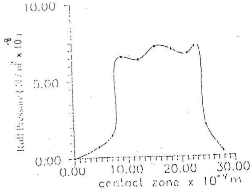
Fig. (2-a) A theoretical pressure distribution for 14 percent reduction of steel strip using oil H (Dow et al, 1975)
