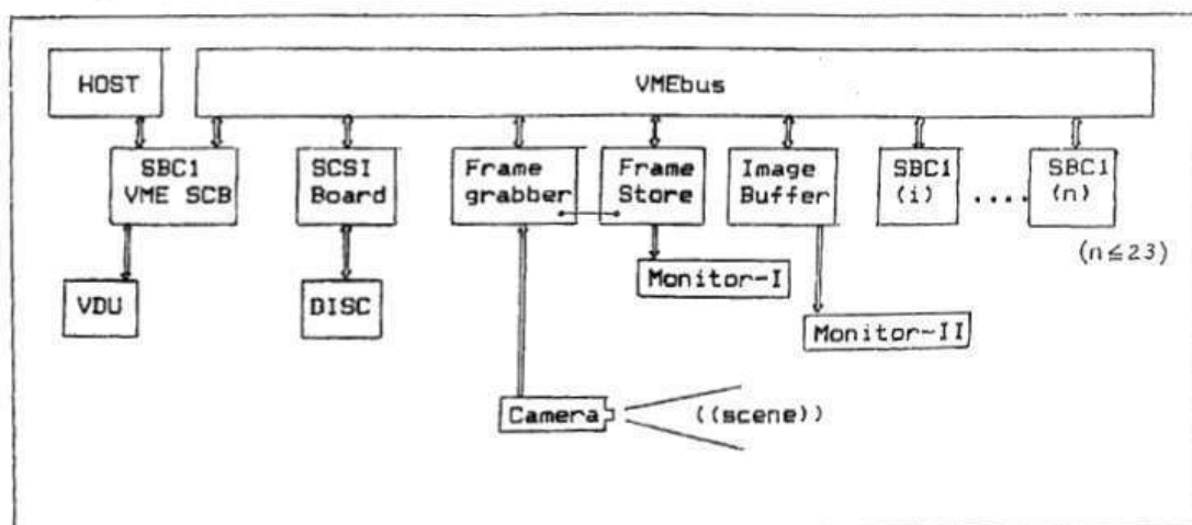
Fig.(4) System Hardware Configuration
