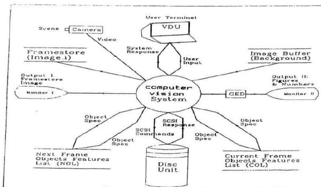
Fig.(3) System Context Diagram (GED = Graphics Editor)
