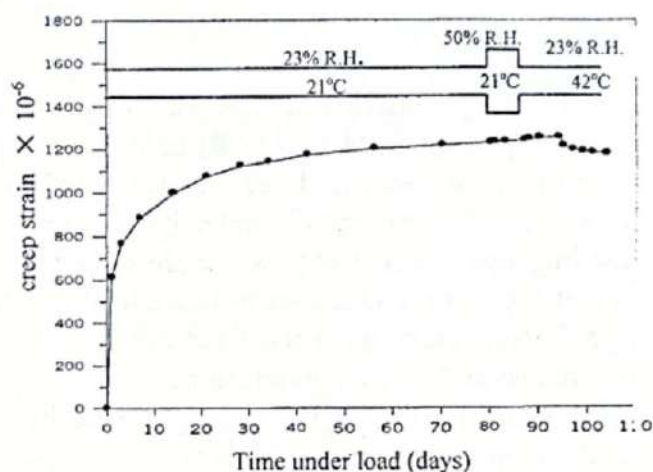
Fig. (3) Observed creep strain vs. time under load for series (1).
