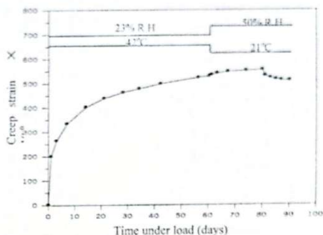
Fig. (5) Observed creep strain vs. time under load for series (2).
