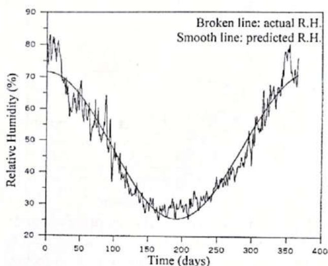
Fig. (15) Actual and predicted relative humidity vs. time throughout a year, starting on the first of January.
