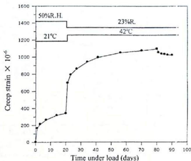
Fig.(7) Observed creep strain vs. time under load for series (3).
