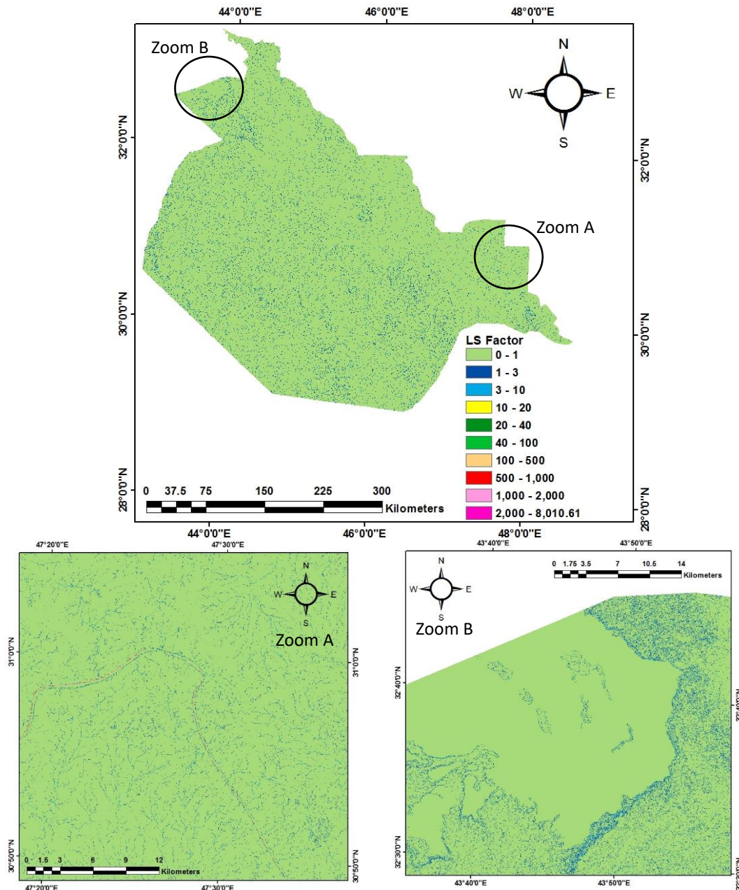
Fig. 5. Topographic factor LS map of Euphrates watershed.
