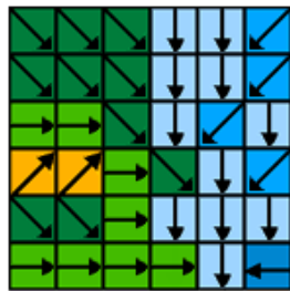
Fig. 3A. Flow direction
