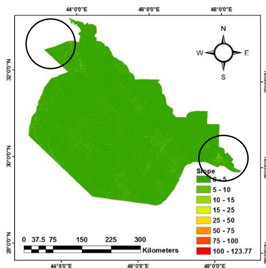
Fig. 4A. Slope percentage map of Euphrates watershed.
