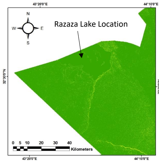
Fig. 4B. slope percentage map of Razaza lake.
