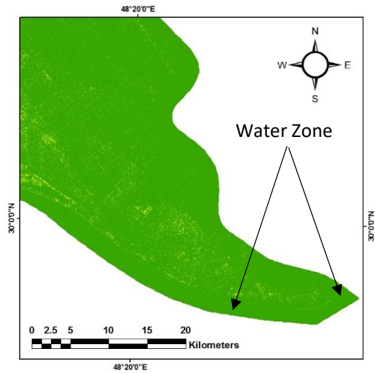
Fig. 4C. slope percentage map of Fao city.
