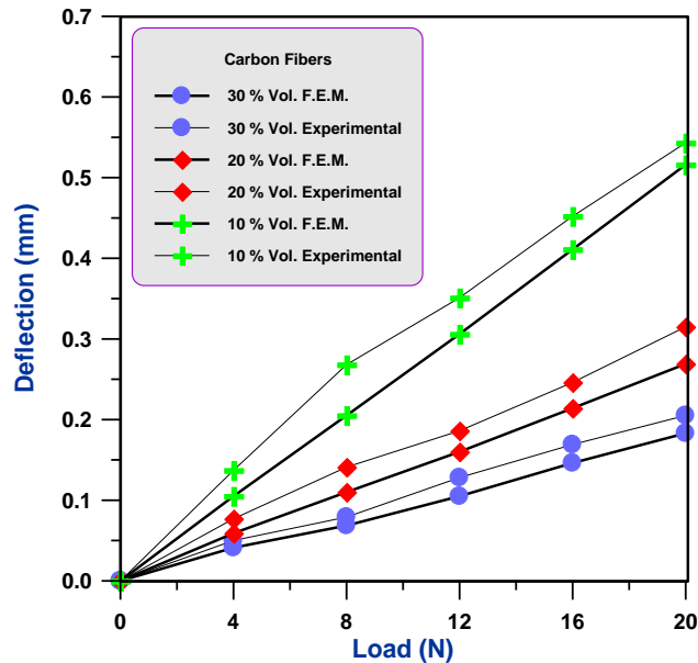
Figure (6): Load Deflection Of The Composite Beam Reinforced By Garbon Fibers Experimental And F.E. Analysis.
