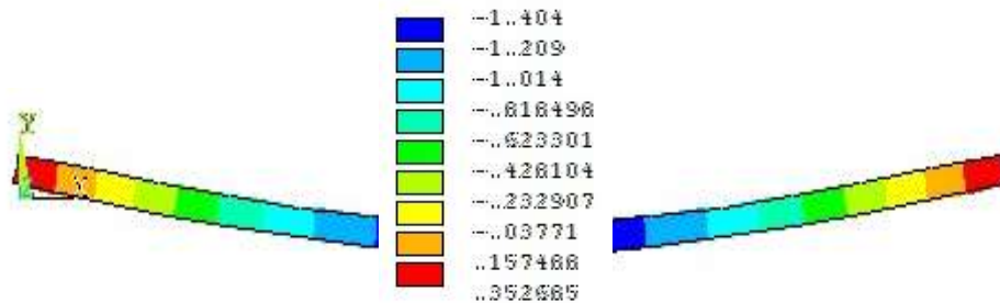
Figure (4) Sample Of Deflection Contours Of Composite Beam When Reinforced By Glass Fibers At ( V_f = 10\% ) And Load ( =20\text{ N} ).
