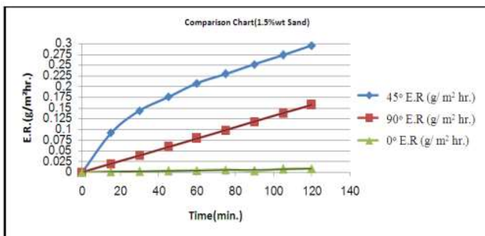
Figure (4) Variation of erosion rate of Al alloy with time (Different impact angle, 1.5% sand).
