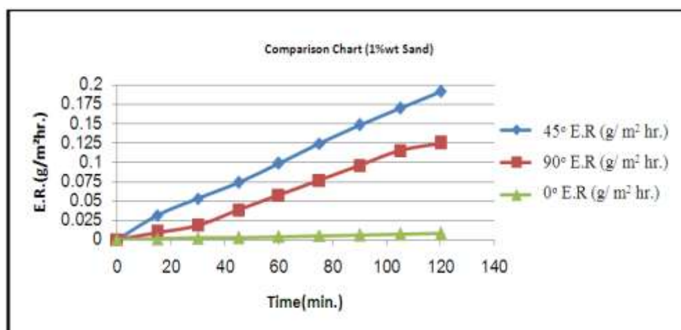
Figure (3) Variation of erosion rate of Al alloy with time (Different impact angle, 1% sand).
