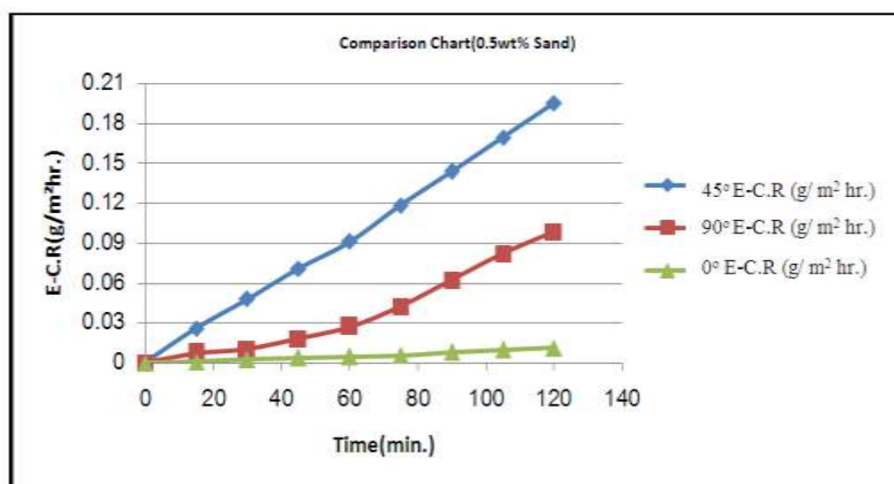
Figure (5) Variation of erosion-corrosion rate of Al alloy with time (Different impact angle, 0.5% sand).
