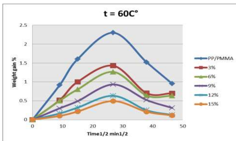
Figure (9) Relation between weight gain % and time 1/2 of PP/PMMA/unfilled/filled with different weights and particle sizes of BN at 45 \mu\text{m} at t = 60\text{C}^\circ .
