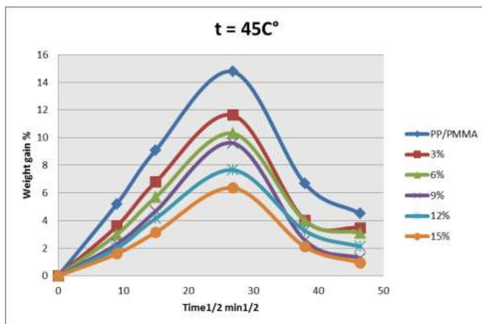
Figure (8) Relation between weight gain % and time 1/2 of PP/PMMA/unfilled/filled with different weights and particle sizes of BN at 45 \mu\text{m} at t = 45\text{C}^\circ .
