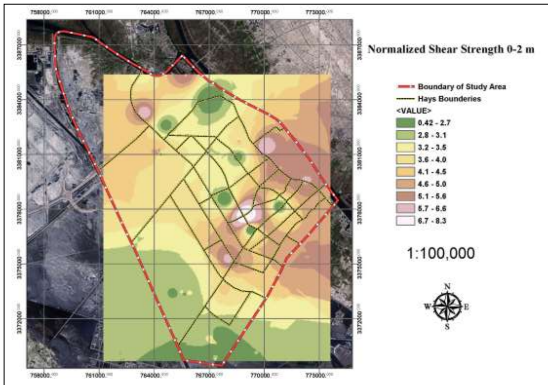
Figure (9) Distribution of normalized shear strength at depth 0-2 m across study area.
