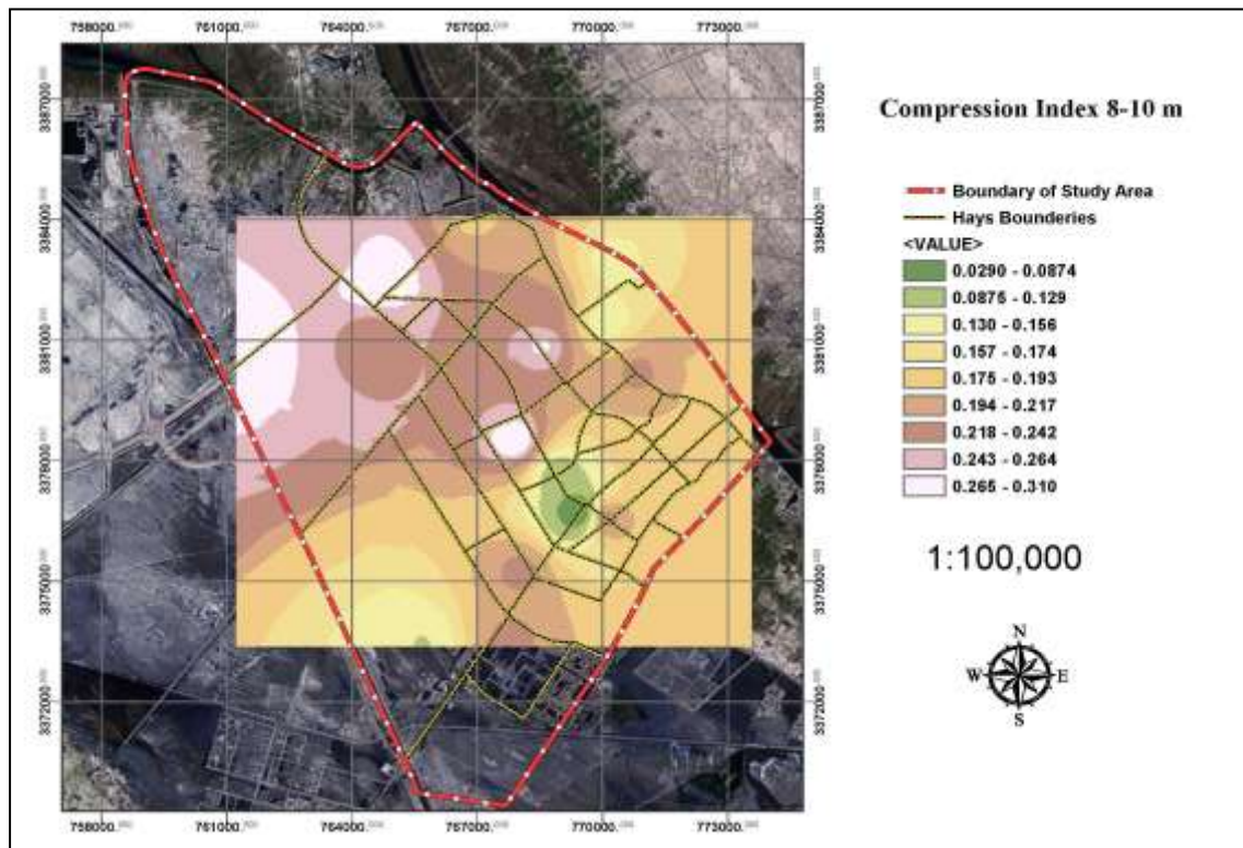
Figure (23) Distribution of compression index at depth 8-10 m across study area.
