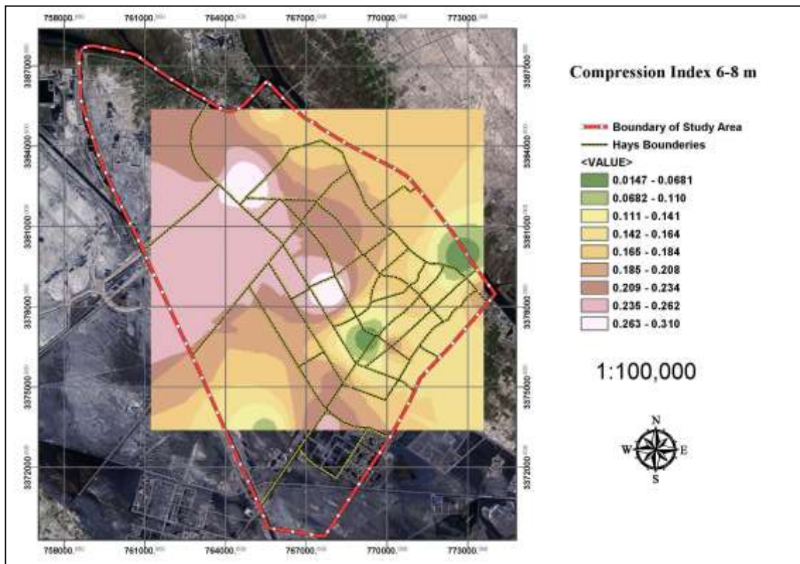
Figure (22) Distribution of compression index at depth 6-8 m across study area.
