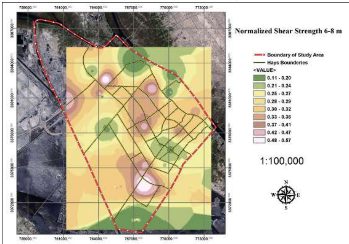
Figure (12) Distribution of normalized shear strength at depth 6-8 m across study area.
