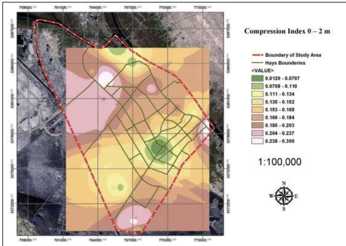
Figure (19) Distribution of compression index at depth 0-2 m across study area.
