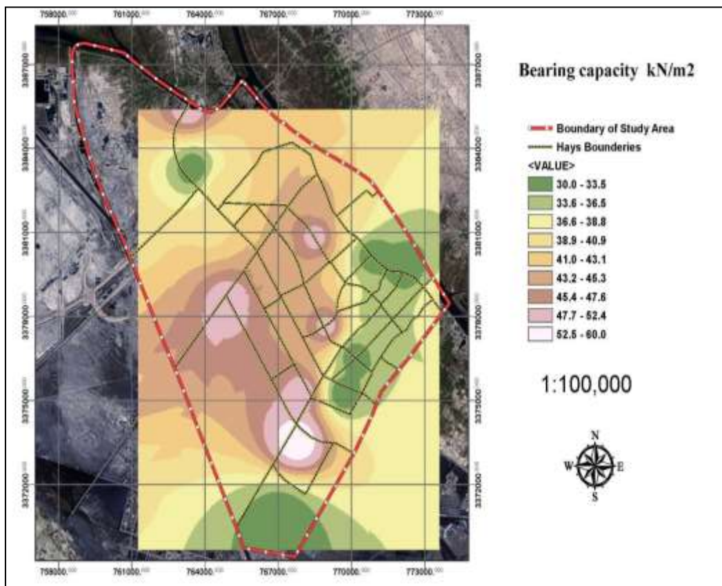
Figure (8) Bearing capacity distribution across study area.
