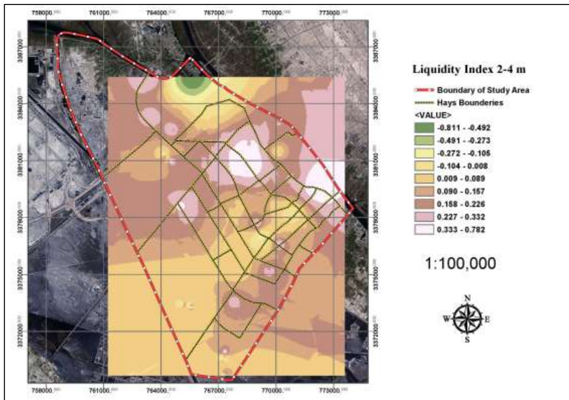
Figure (15) Distribution of liquidity index at depth 2-4 m across study region
