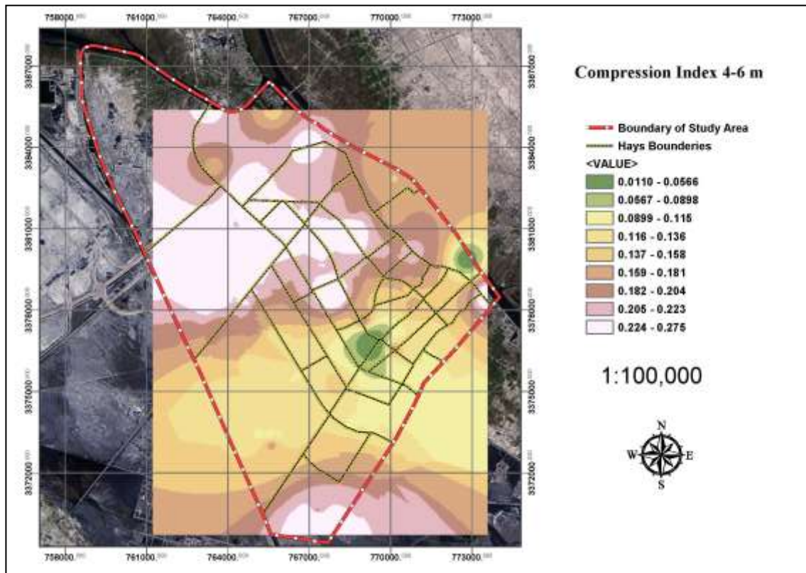
Figure (21) Distribution of compression index at depth 4-6 m across study area
