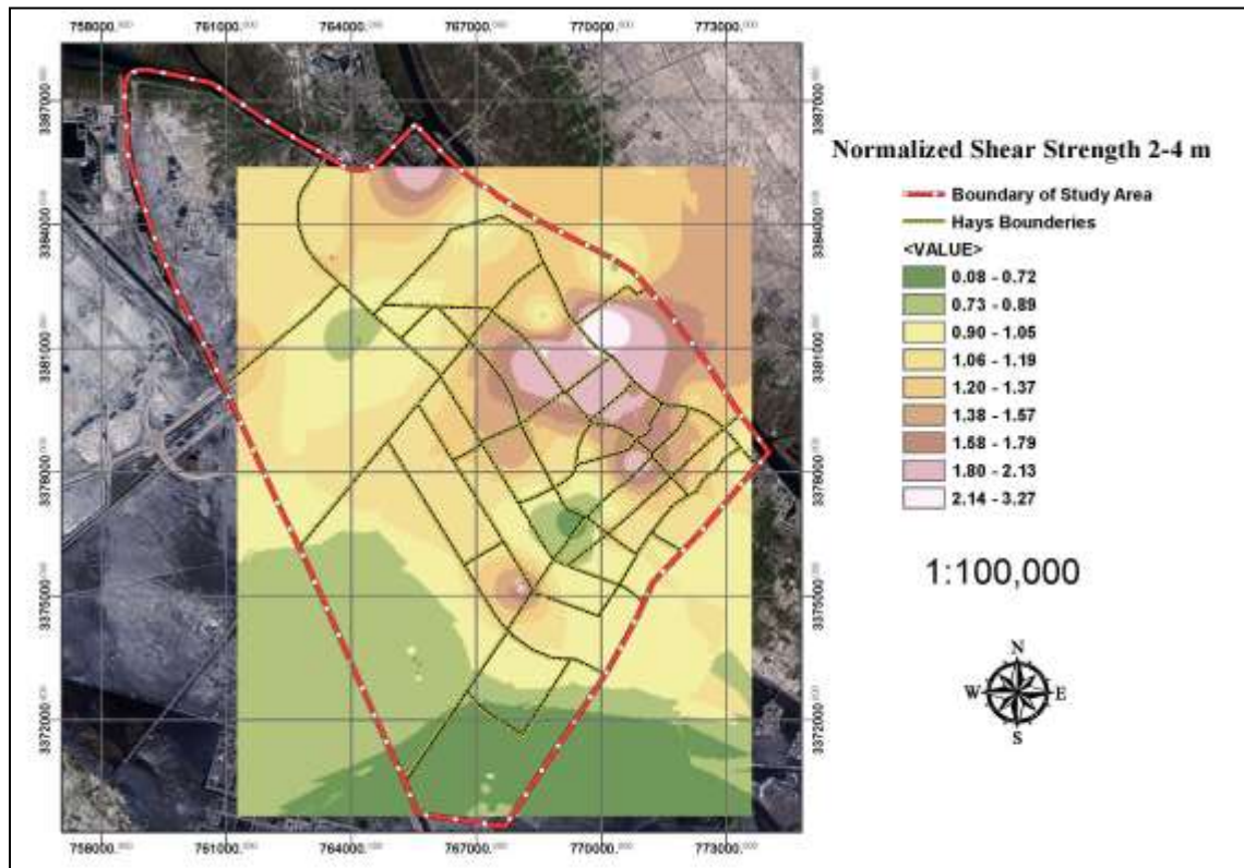
Figure (10) Distribution of normalized shear strength at depth 2-4 m across study area.
