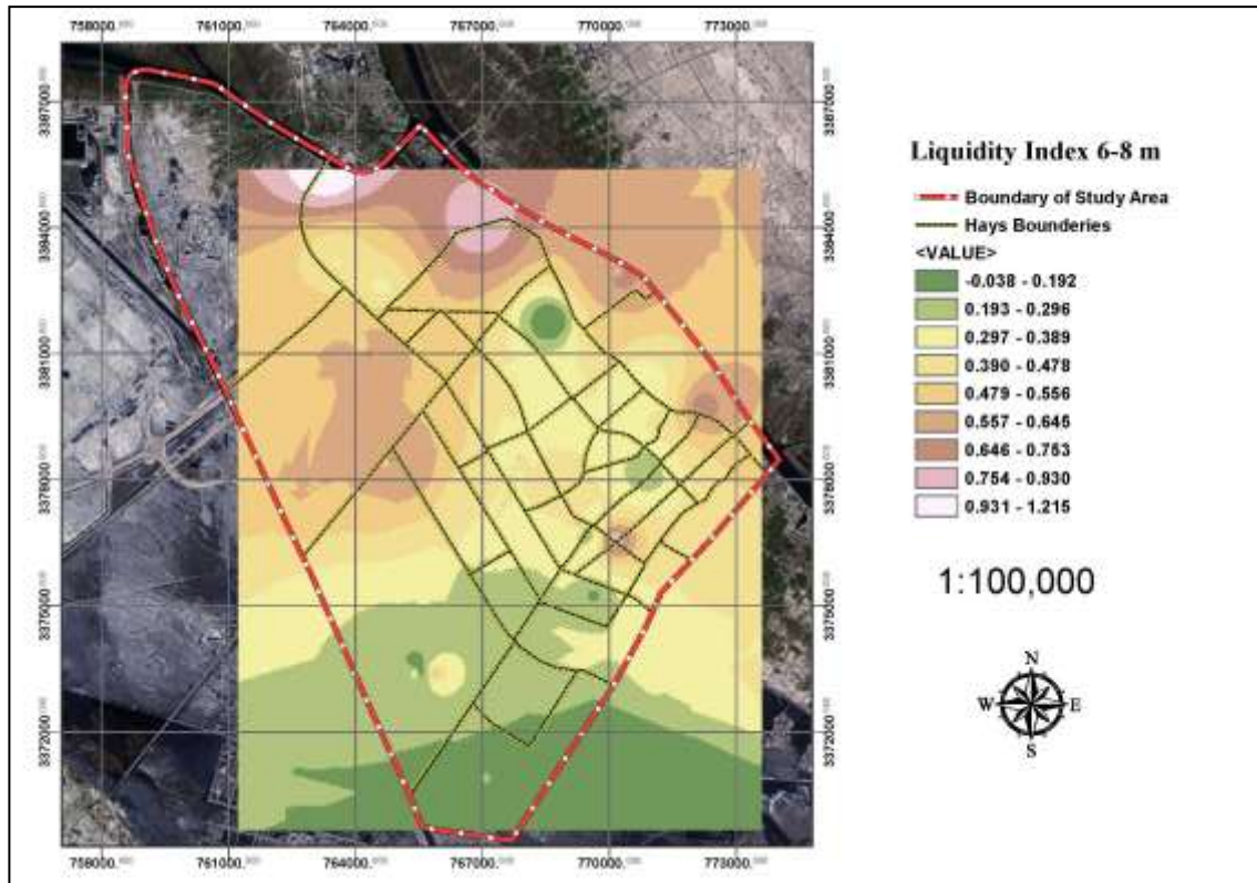
Figure (17) Distribution of liquidity index at depth 6-8 m across study region.
