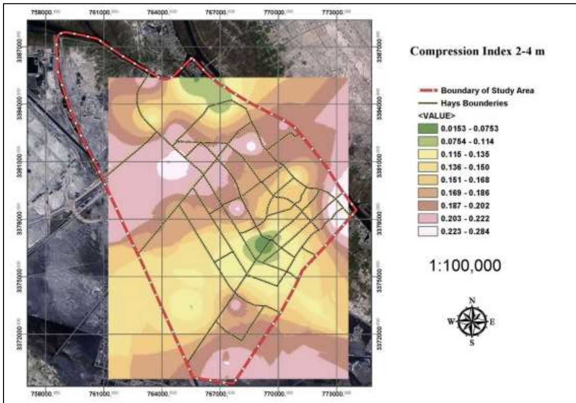
Figure (20) Distribution of compression index at depth 2-4 m across study area.
