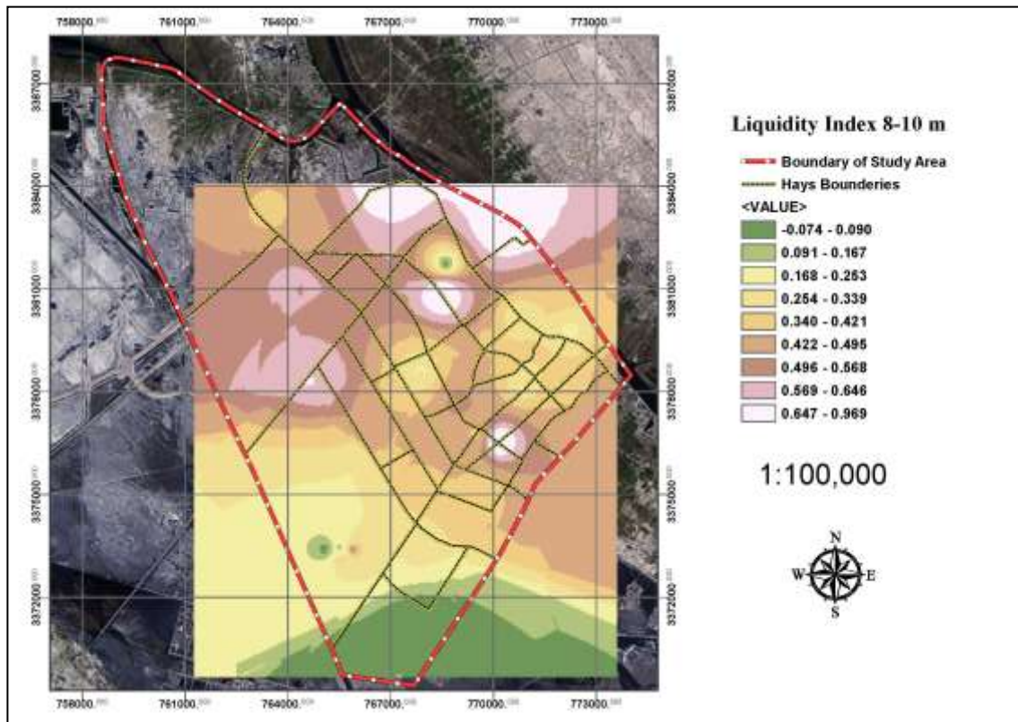
Figure (18) Distribution of liquidity index at depth 8-10 m across study region
