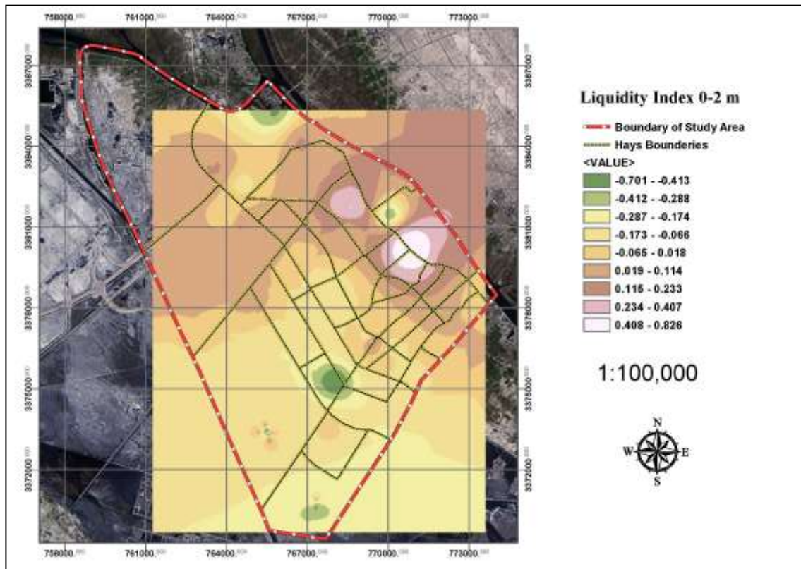
Figure (14) Distribution of liquidity index at depth 0-2 m across study region
