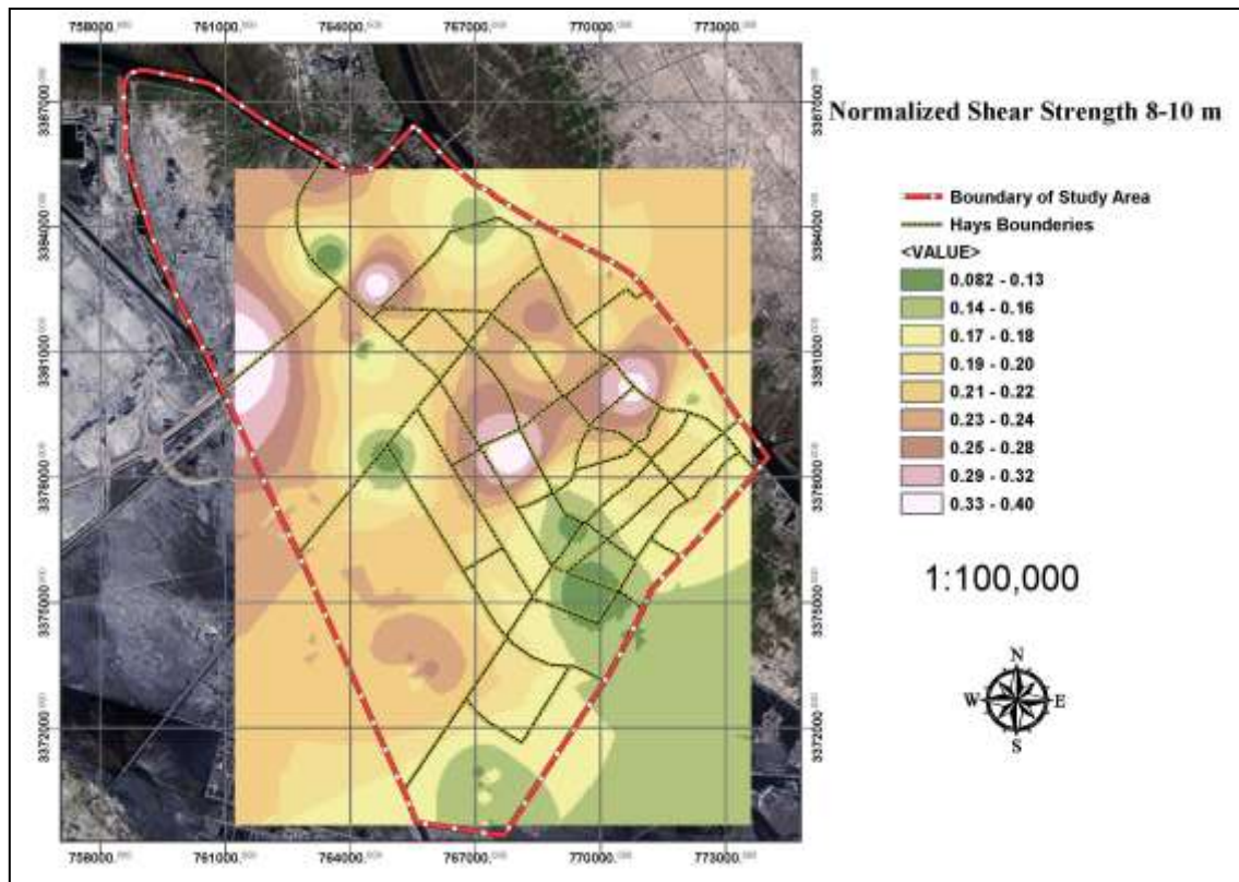
Figure (13) Distribution of normalized shear strength at depth 8-10 m across study
