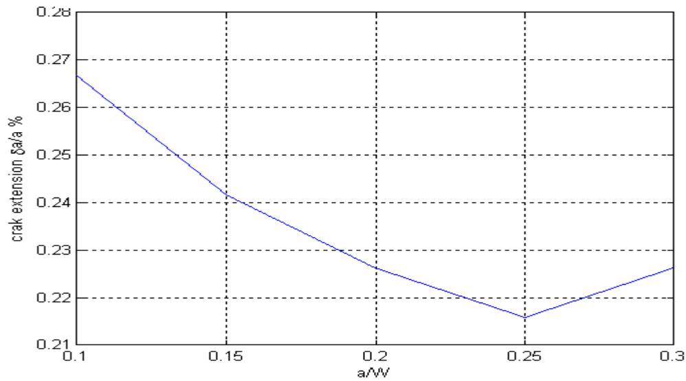
Figure(7)Crack Extention Design Curve for Cental Cracked Plate.
