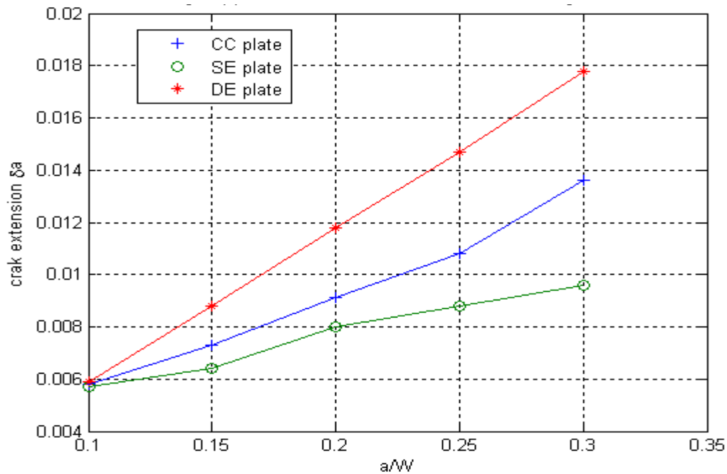
Figure(8) Crack Extention for different Crack onfiguration Plate.
