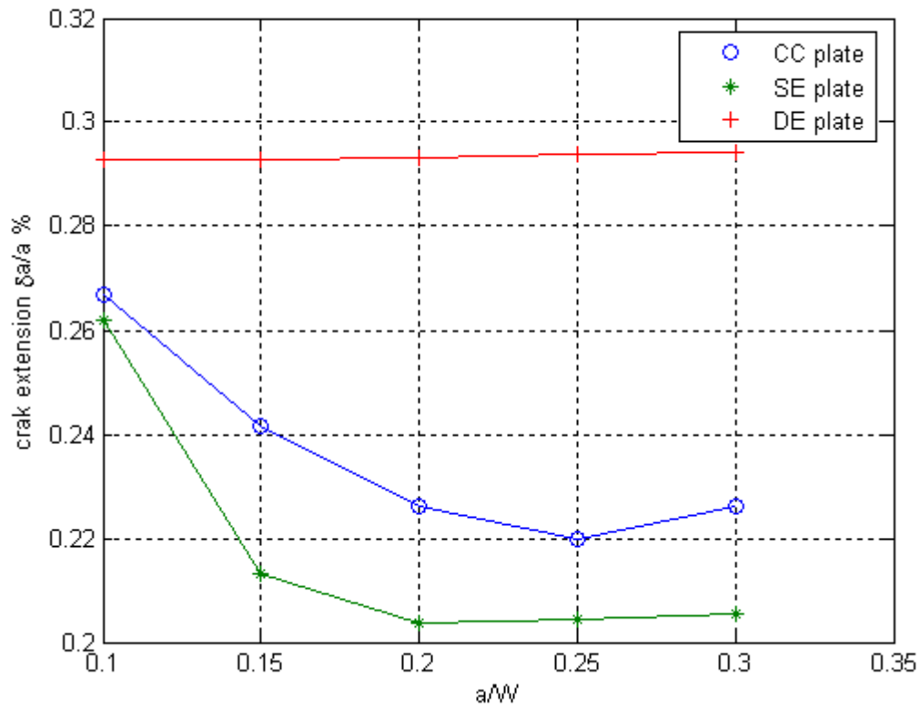
Figure(9)Crack Extension Design Curve for different crack configuration.
