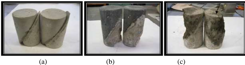
Figure (3) Failure of the composite slant sections [17]. (a) Interface failure, (b) Substrate concrete failure, (c) Repairing material failure.
