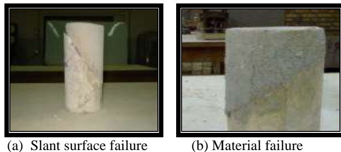
Figure (4) Failure of the composite slant sections of the research.
